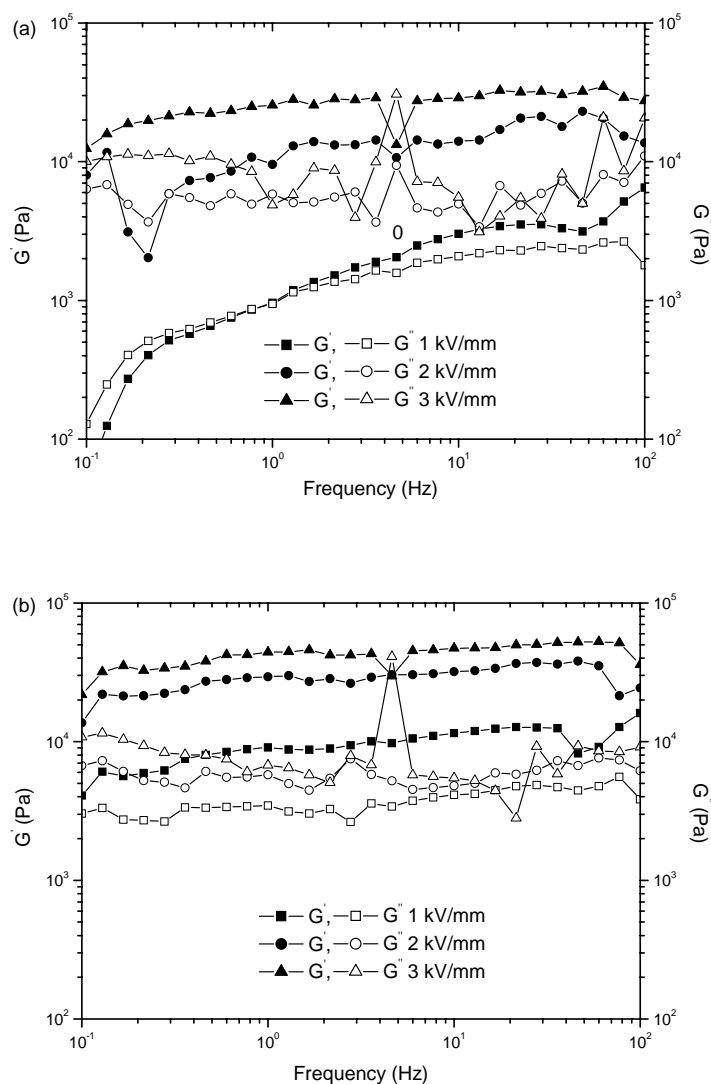
Fig. S4 Frequency dependence of storage modulus ( G' , solid dots) and loss modulus ( G'' , open dots) for suspensions of pure titania particles: (a) smooth; (b) hierarchical. ( T=23\text{ }^{\circ}\text{C} , 10 vol%, Applied stress=10 Pa).
