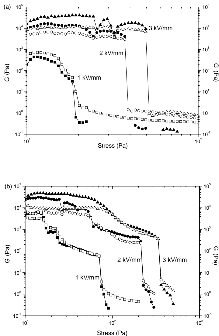
Fig. S5 Stress dependence of storage modulus ( G' , solid dots) and loss modulus ( G'' , open dots) for suspensions of pure titania particles: (a) smooth; (b) hierarchical. (T=23 °C, 10 vol%, Applied frequency=0.5 Hz).
