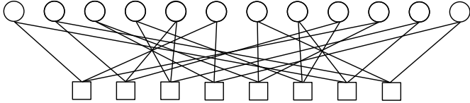
Fig. 2. Sample QC-LDPC PCM and associated graph
