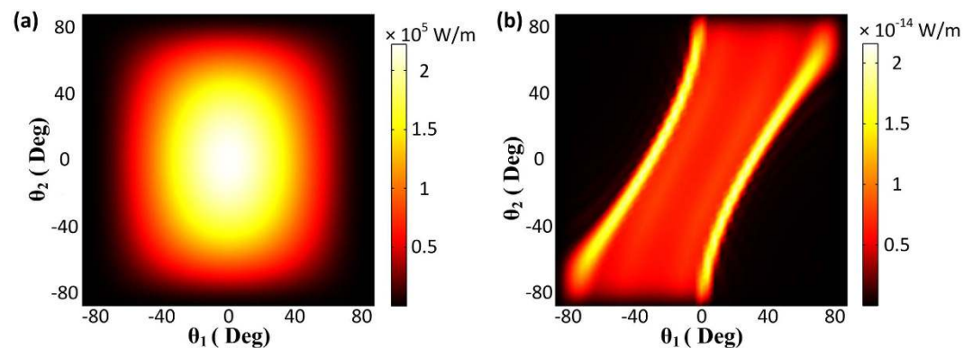
Figure 4. Power outflow of the generated FWM wave as a function of the incident angles of both excitations for (a) the nonlinear metasurface and (b) the bare silver film. The generated FWM power outflow of the nonlinear metasurface is enhanced, homogeneous and relatively insensitive to the incident angles compared to a bare silver film.
