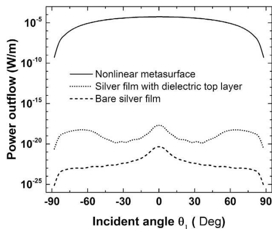
Figure 6. Power outflow of the generated 13.5 THz FWM wave as a function of different excitation angles for the nonlinear metasurface (solid line), a silver film with a nonlinear dielectric top layer (dotted line) and a bare silver film (dashed line). The incident wavelengths of the pump waves are \lambda_1 = 1206 nm and \lambda_2 = 620 nm and the wavelength of the generated low-THz FWM wave is \lambda_3 = 22 \mu m. The power outflow of the generated 13.5 THz FWM wave is enhanced by fifteen orders of magnitude compared to a bare silver film.
