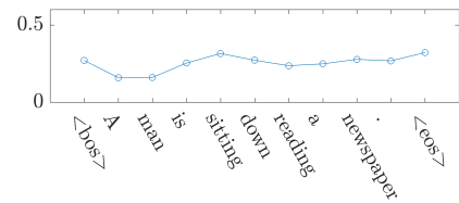
(e) Input gate of BiLSTM in inference composition ( l^2 -norm)
