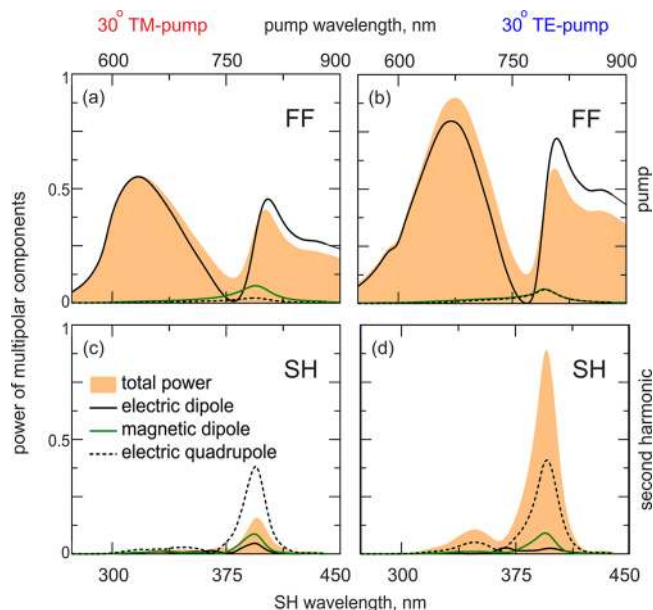
Figure 4. Numerically calculated cross sections of the electric dipole (black, solid), electric quadrupole (black, dashed), and magnetic dipole (green) at (a, b) fundamental wavelengths and (c, d) second-harmonic wavelengths, for two polarizations of the pump at the oblique incidence.
