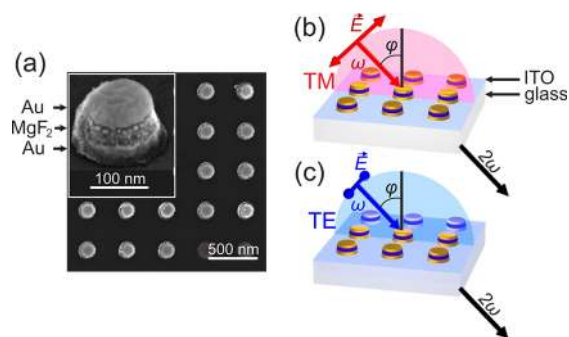
Figure 1. (a) SEM image of a fabricated metasurface. Inset shows a side view of a single three-layer meta-atom made of Au/MgF 2 /Au layers. (b, c) Geometry of the SHG experiment for TM- and TE-polarized pump waves, respectively.
