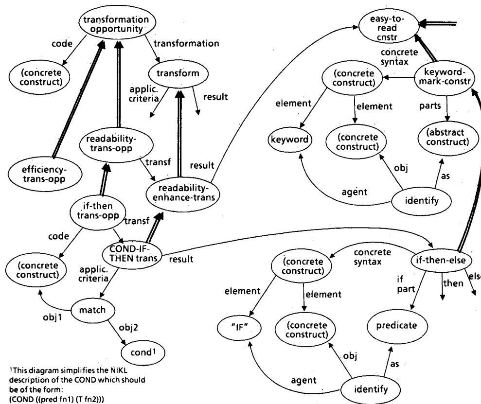
Fig. 7. Simplified NIKL representation of IF-THEN-ELSE transform.
