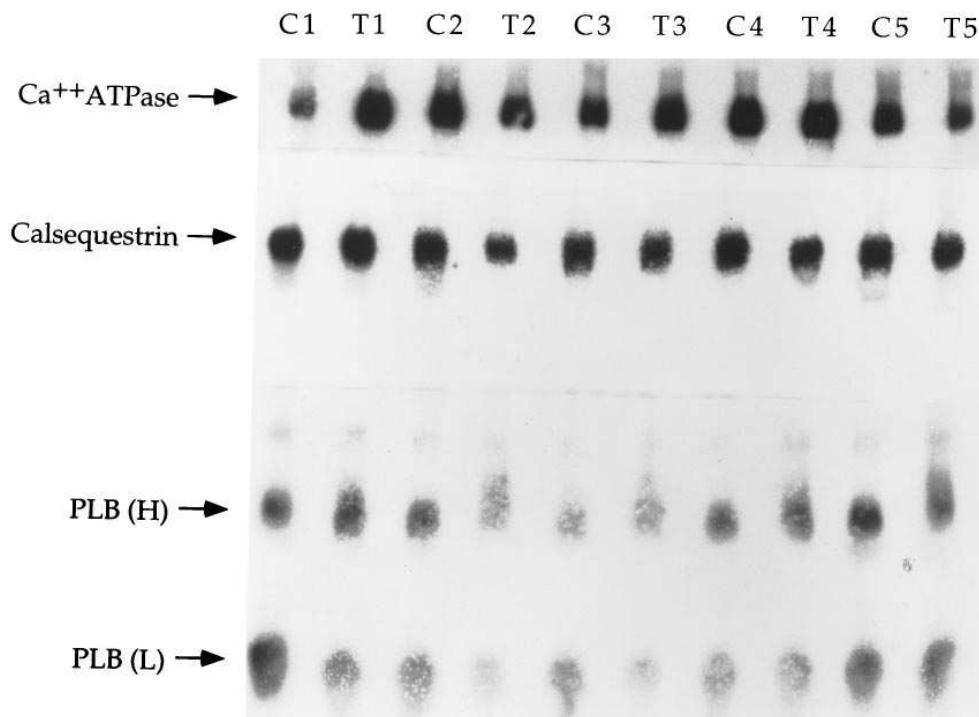
Figure 5. SR \text{Ca}^{2+} ATPase, calsequestrin, and phospholamban (PLB) immunoreactivity in hearts from control ( C , n = 5 ) and transgenic ( T , n = 5 ) mice showing the selective reduction in phospholamban with targeted \beta_2 -AR stimulation. The autoradiograph of the nitrocellulose sheet is shown. Radioactivity was quantified with use of a GS-250 Molecular Imaging System (Bio-Rad Laboratories). Densitometric quantification of the various autoradiograms, control vs. transgenic (arbitrary units): SR \text{Ca}^{2+} ATPase 0.97 \pm 0.26 vs. 1.23 \pm 0.34 , P = \text{NS} ; calsequestrin 0.95 \pm 0.08 vs. 0.78 \pm 0.06 , P = \text{NS} ; PLB 1.11 \pm 0.06 vs. 0.85 \pm 0.08 , P = 0.025 . Both high ( H ) and low ( L ) molecular weight forms of PLB were used in the quantification (see text).
