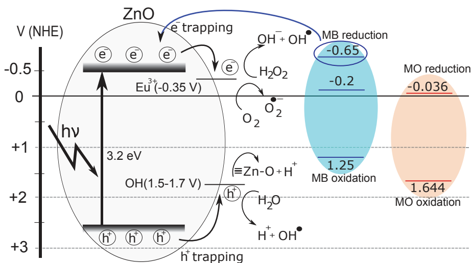
Fig. 9. Scheme of the energy levels in Eu 3+ doped ZnO with possible photocatalytic mechanism of MB and MO degradation.
