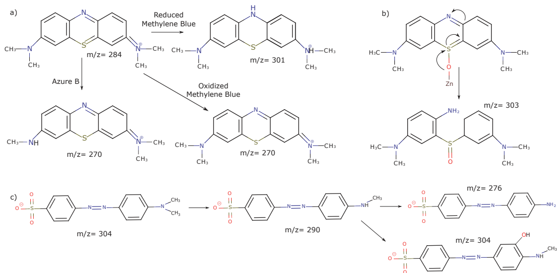
Fig. 12. Possible a) MB degradation path in the presence of \bullet\text{OH} scavenger b) MB degradation path in the presence of hole scavenger c) MO degradation path in the presence of hole scavenger.
