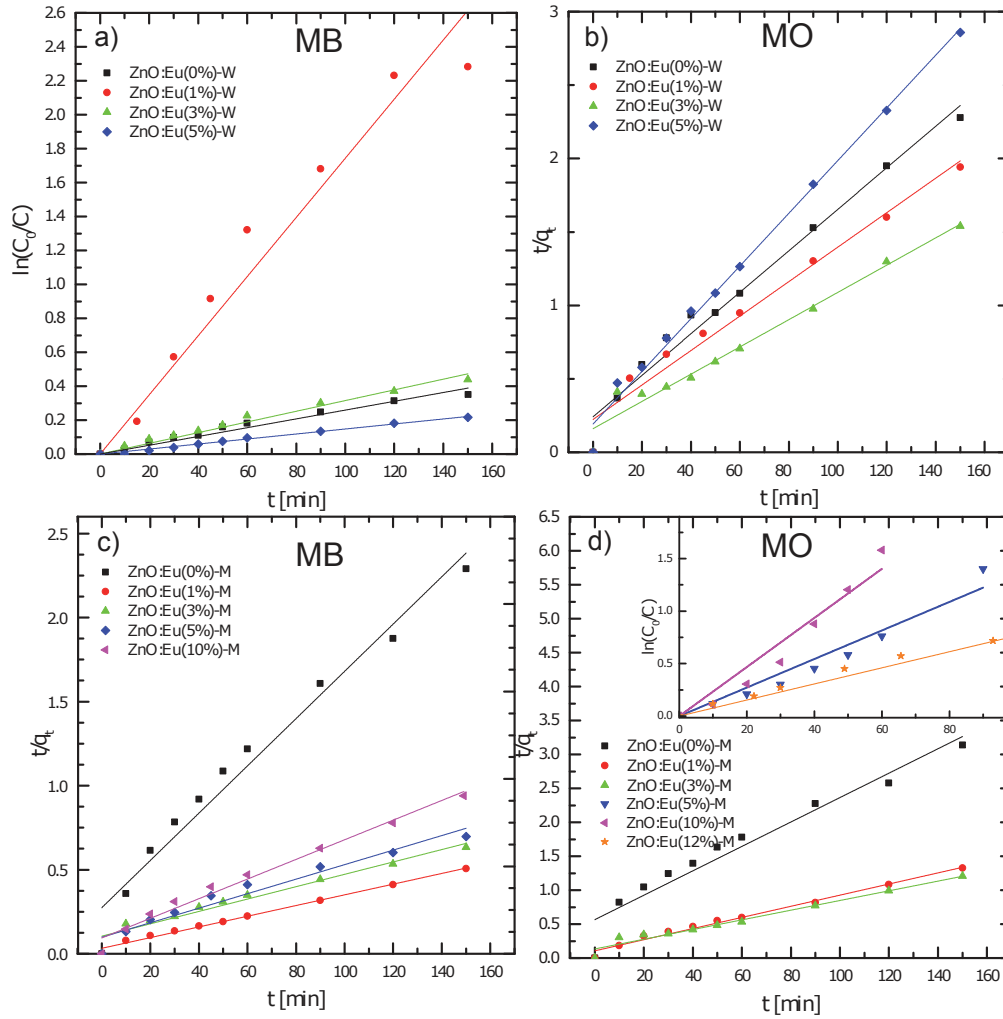
Fig. 8. Pseudo-first-order linear plots of \ln(C_0/C) (figure a and inset in figure d) and pseudo-second-order linear plots of t/q_t (figures b,c and d) versus irradiation time for the degradation kinetics of MB and MO using different photocatalysts.
