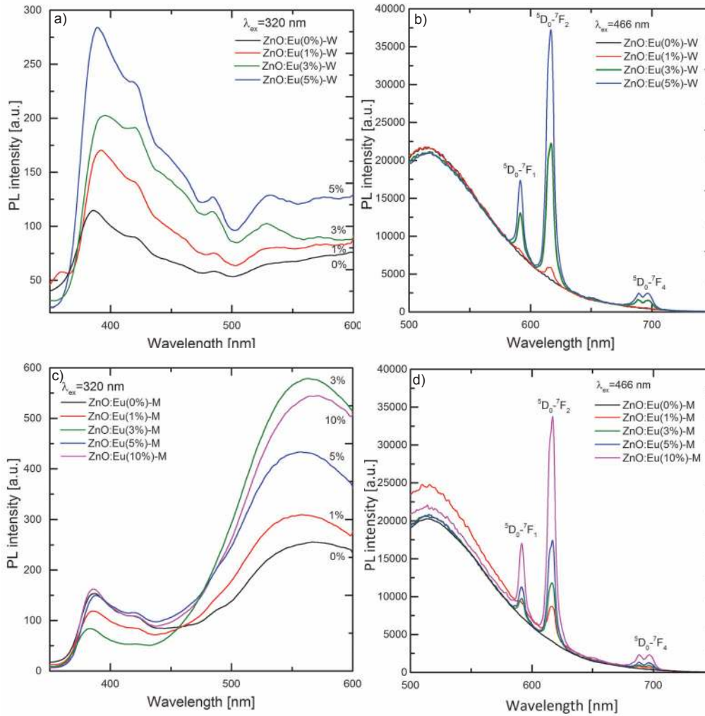
Fig. 4. Room temperature PL emission of a) ZnO:Eu(x%)-W with excitation wavelength \lambda_{ex}=320 nm b) ZnO:Eu(x%)-W, \lambda_{ex}=466 nm, c) ZnO:Eu(x%)-M \lambda_{ex}=320 nm; d) ZnO:Eu(x%)-M \lambda_{ex}=466 nm
