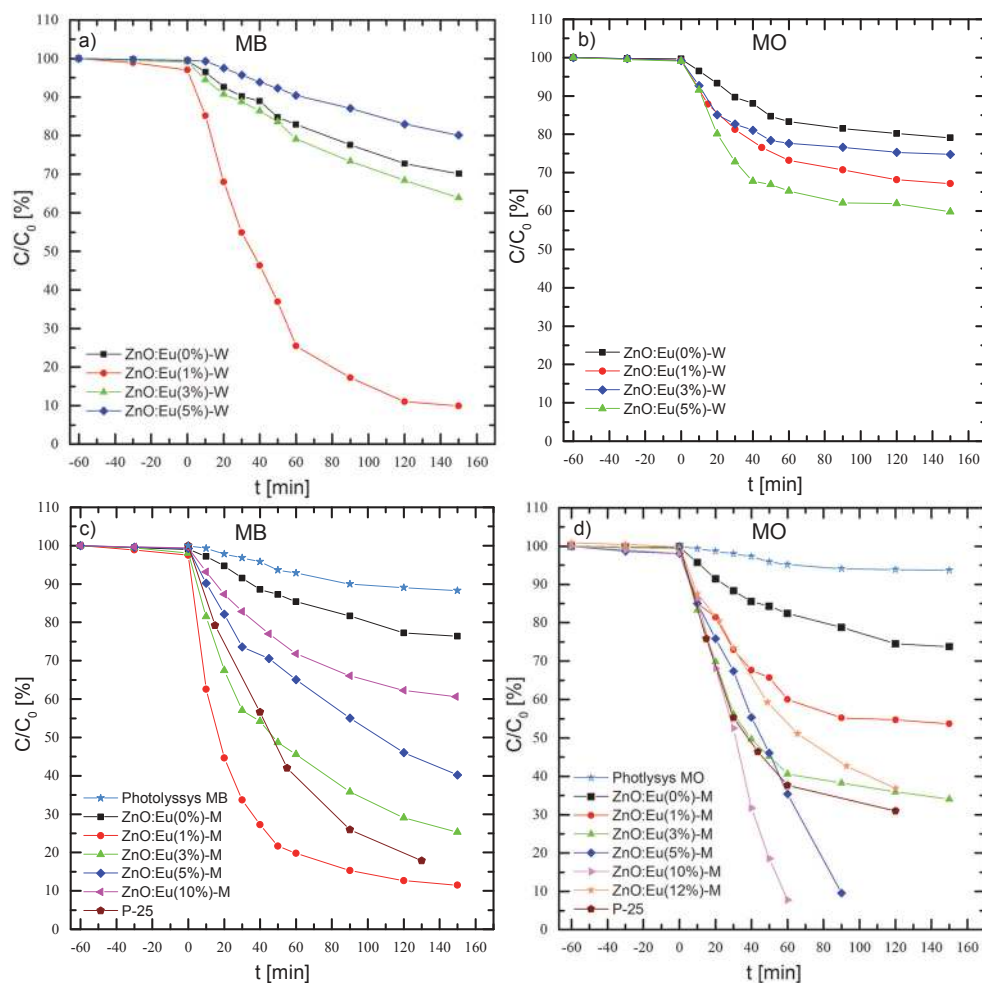
Fig. 7. Effect of \text{Eu}^{3+} doping content in \text{ZnO:Eu}(x\%)\text{-W} on a) MB b) MO; and in \text{ZnO:Eu}(x\%)\text{-M} on c) MB d) MO concentration. Dyes concentration are 10 ppm, photocatalyst amount is 1 mg per 1 ml of dye.
