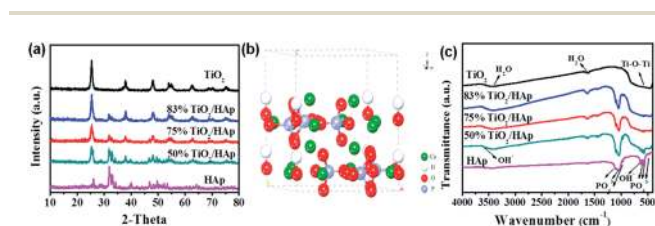
Fig. 1 XRD patterns of as-synthesized samples (a), the crystal structure models of HAp (b) and FTIR spectra of TiO 2 , HAp and TiO 2 /HAp (50%, 75% and 83%) composites (c).
