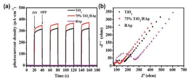
Fig. 6 Transient photocurrent densities (a) and electrochemical impedance spectroscopy measurements (b) of pure \text{TiO}_2 , HAp, \text{TiO}_2/\text{HAp} composite.
