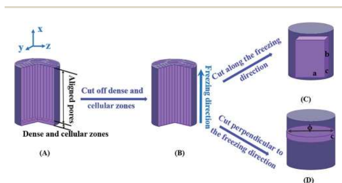
Fig. 1 Schematic of the preparation of the freeze-cast samples. (A) Sintered PZT ceramic, (B) aligned porous PZT sample after removing the dense and cellular zones, (C) cutting along the freezing direction and (D) perpendicular to the freezing direction.
