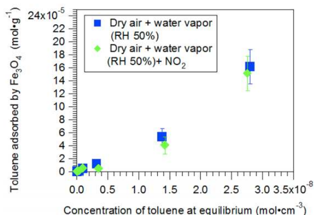
Figure 3. Experimental adsorption isotherms of toluene on magnetite at relative humidity of 50% alone (blue ■) and in the presence of NO 2 (green ◆). Error bars represent standard errors calculated by the propagation of errors during preparation and analyses. Limit of detection is (2.90 \times 10^{-12}) \pm (1 \times 10^{-15}) mol·cm -3 .
