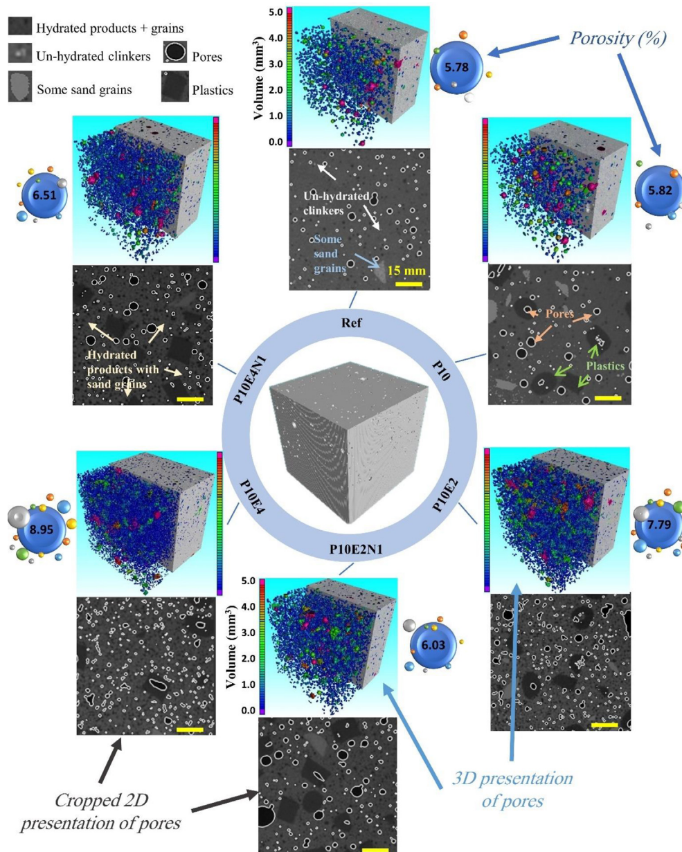
Fig. 7. 2D and 3D \mu -XCT images of the Ref at the top, and going clockwise for other specimens in order: P10, P10E2, P10E2N1, P10E4, and P10E4N1. Air voids are demonstrated in the 3D \mu -XCT images based on their volumes. Porosities are indicated in circles besides each 3D image.
