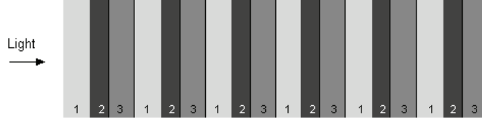
Figure 1. Structure of one-dimensional ternary photonic crystal sensing element.
