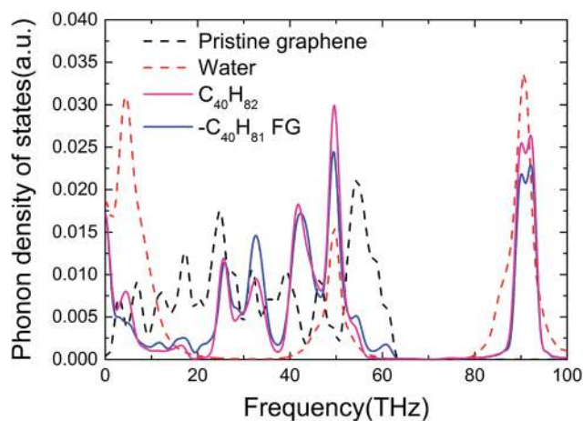
Fig. 4 Phonon DOSs of pristine graphene, water, -C_{40}H_{81} functionalized graphene and the corresponding functional group in stable state ( C_{40}H_{82} ). The functionalized alkane alters the phonon vibration modes of graphene dramatically.
