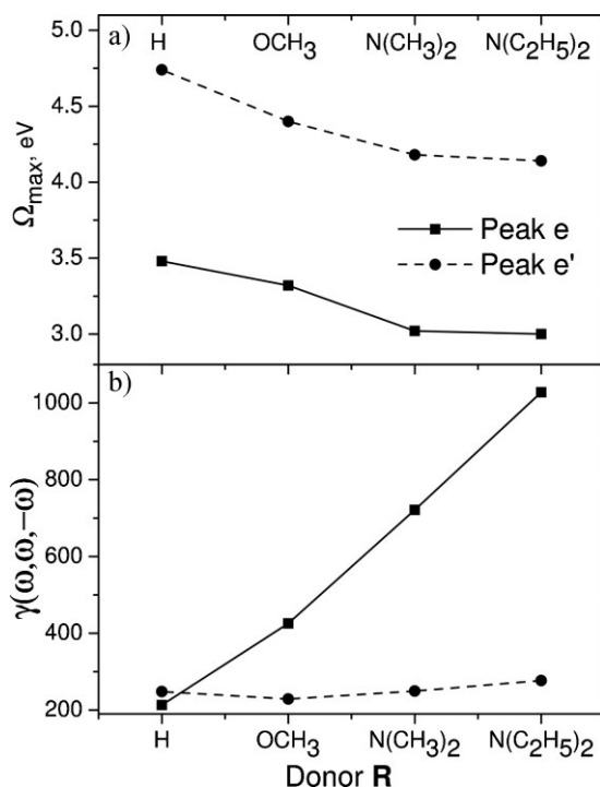
Figure 10. Variation of third-order polarizabilities (all \gamma are given in 10^{-32} esu) with the strength of the terminal donor groups for compounds q_4 – q_7 in Figure 7. The lines connecting the points serve as a visual guide. Adapted from [194].
