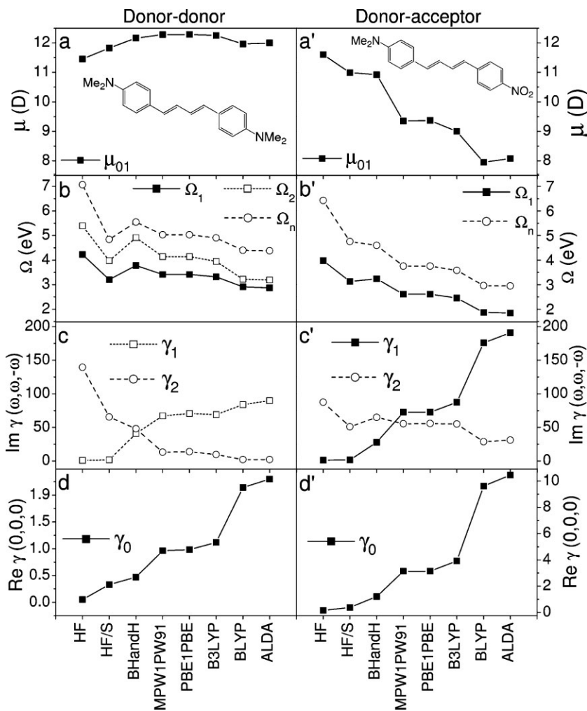
Figure 3. Transition dipoles between the ground and first excited states (a and a'), transition energies between the ground and excited states contributing to NLO response (b and b'), resonant (c and c') and static (d and d') third-order polarizabilities (all \gamma are given in 10^{-33} esu) as a function of DFT model used for calculations. Adapted with permission from [193], copyright 2004 Elsevier.
