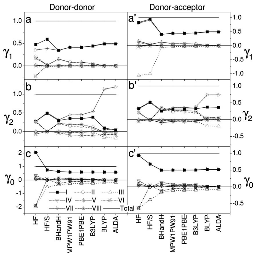
Figure 5. Relative contributions from different terms in Equation 47 to resonant (a, a' and b, b') and static (c and c') NLO responses as a function of DFT model. Adapted with permission from [193], copyright 2004 Elsevier.
