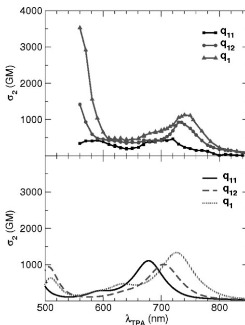
Figure 13. TPA cross section of chromophores q_1 , q_{11} , and q_{12} . Top panel: experimental data in toluene; Bottom panel: calculated cross section in vacuum, but corrected for local field and refractive index. Adapted from [126].
