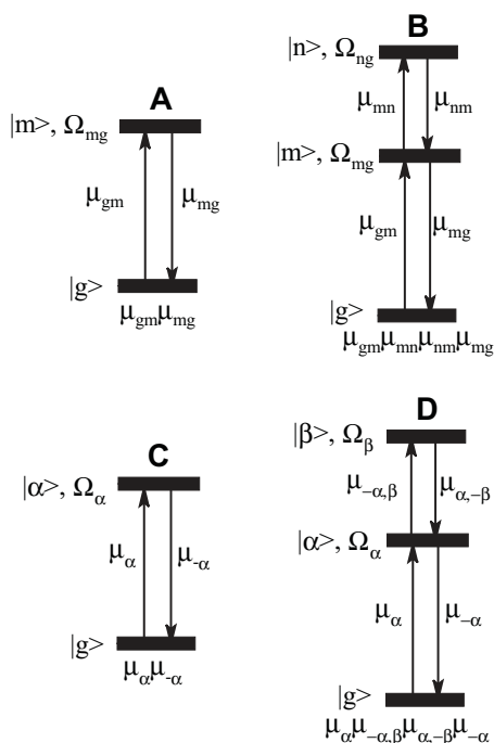
Figure 2. A,B) Representation of the SOS for the first- and third-order responses (Eqs. 39 and 40) in terms of Liouville space pathways. C,D) Similar interpretation of TD-DFT response expressions (Eqs. 46 and 47), adapted with permission from [182].
