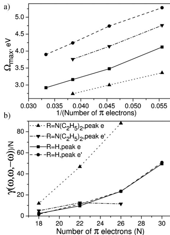
Figure 11. Variation of third-order polarizabilities (all \gamma are given in 10^{-32} esu) with the number of \pi -electrons roughly representing the length of the \pi -bridge for compounds q_2 , q_4 , q_8 , q_{10} ( R=H ), and q_3 , q_6 , q_9 ( R=N(C_2H_5)_2 ) in Figure 7. The lines connecting the points serve as a visual guide. Adapted from [194].
