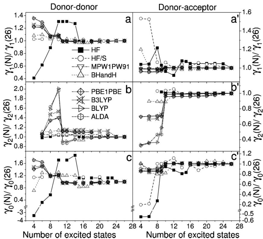
Figure 4. Variation of magnitudes of resonant polarizabilities at the first (a and a') and second (b and b') TPA maxima, and static polarizability (c and c') with the number of excited states used for calculations. Adapted with permission from [193], copyright 2004 Elsevier.
