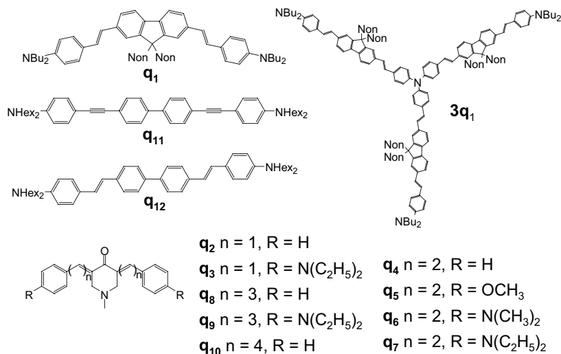
Figure 7. Molecular structure of quadrupolar compounds q_1 – q_{12} and branched chromophore 3q_1 . Index n denotes the number of vinyl units (i.e., the number of double bonds in the conjugated bridge) for the arylidencyclohexanone chromophores q_2 – q_{10} .
