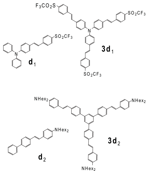
Figure 6. Molecular structures of dipolar chromophores d_1 and d_2 , and three-branched octupolar compounds 3d_1 and 3d_2 .
