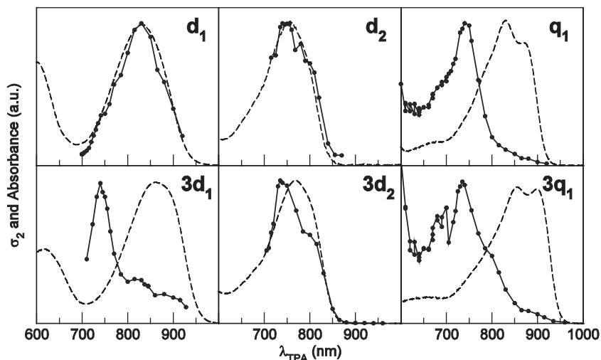
Figure 19. Experimental TPA (circles and lines) and rescaled OPA (dashed lines) spectra for monomeric compounds d_1 , d_2 , and q_1 , and their corresponding branched systems 3d_1 , 3d_2 , and 3q_1 in toluene.
