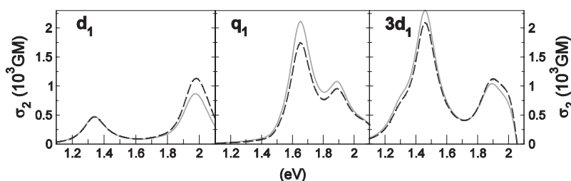
Figure 9. Effect of local-field and refractive-index corrections on TPA cross sections of dipolar ( d_1 ), quadrupolar ( q_1 ) and 3-branched octupolar ( 3d_1 ) chromophores obtained using the tol-tol (“single point-optimization level”) model to calculate second-order hyperpolarizability ( \gamma^{sol} ): no local-field correction (continuous line), local-field correction according to Equation 38 (dashed line).
