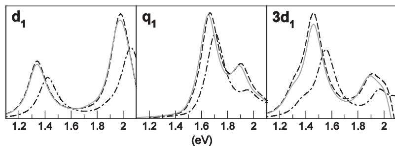
Figure 8. TPA cross sections (arbitrary units) of dipolar ( d_1 ), quadrupolar ( q_1 ) and 3-branched octupolar ( 3d_1 ) chromophores obtained with different models for the second-order hyperpolarizability ( \chi^{(2)} ): vac-vac (dashed-dotted line), vac-tol (dashed line) and tol-tol (continuous line) (see main text).
