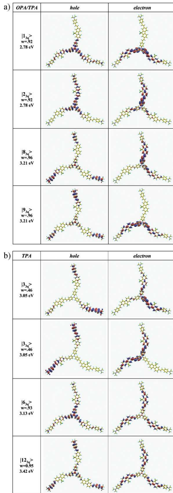
Figure 17. Natural transition orbitals [281] of chromophore 3q_1 . Left panels quote in sequence excited state number, associated NTO eigenvalues [306] and transition energies. Adapted from [126].
