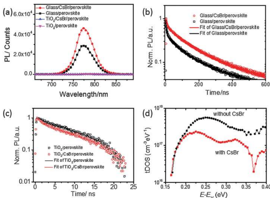
Fig. 3 (a) Steady-state photoluminescence spectra of perovskite thin films deposited on glass and c\text{-TiO}_2 layer with and without CsBr modification collected following excitation at 510\text{ nm} , (b) time-resolved photoluminescence spectra of perovskite thin films on glass collected at 400\text{ kHz} (c) and on c\text{-TiO}_2 layer collected at 30\text{ MHz} at 0.03\ \mu\text{J per cm}^2 per pulse, (d) trap density of states (tDOS) for devices without CsBr (black) and with CsBr modification (red).
