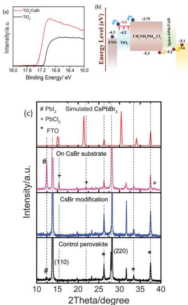
Fig. 2 (a) UPS spectra of c -TiO 2 with (w) and without (w/o) CsBr modification. The light source of UPS is a He1 discharge lamp ( h\nu = 21.2 eV); (b) energy level diagram of the device with the structure of FTO/ c -TiO 2 (CsBr)/perovskite/spiro-OMeTAD/Au; (c) X-ray diffraction spectra of control perovskite on c -TiO 2 (black line), perovskite on c -TiO 2 with thin CsBr modification layer (blue line), perovskite on c -TiO 2 with thick CsBr modification layer (pink line) and simulated XRD data for bulk CsPbBr 3 material (red line).
