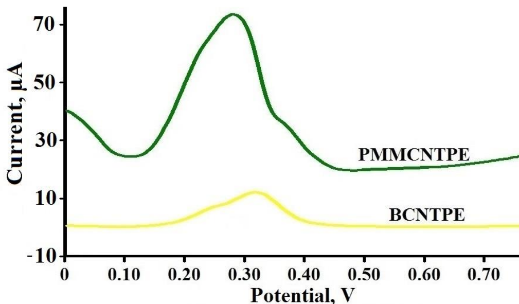
Figure 8. DPVs recorded for 1.0 \times 10^{-4} M PC at BCNTPE and PMMCNTPE in 0.2 M PBS of pH 7.5, at the sweep rate 0.1 \text{ V s}^{-1} .
