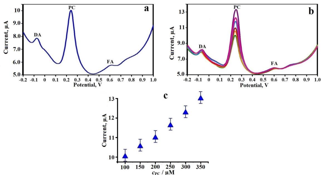
Figure 10. DPVs of PMMCNTPE in 0.2 M PBS of pH 7.5, recorded at the scan rate 0.1 \text{ V s}^{-1} for simultaneous detection of PC, DA and FA at: (a) PC ( 1 \times 10^{-4} \text{ M} ), DA ( 1 \times 10^{-4} \text{ M} ) and FA ( 1 \times 10^{-4} \text{ M} ) (b) DA ( 1 \times 10^{-4} \text{ M} ), FA ( 1 \times 10^{-4} \text{ M} ) and PC varied from 1 \times 10^{-4} - 3.5 \times 10^{-4} \text{ M} , (c) Graphical plot of I_{pa} vs. concentration of PC
