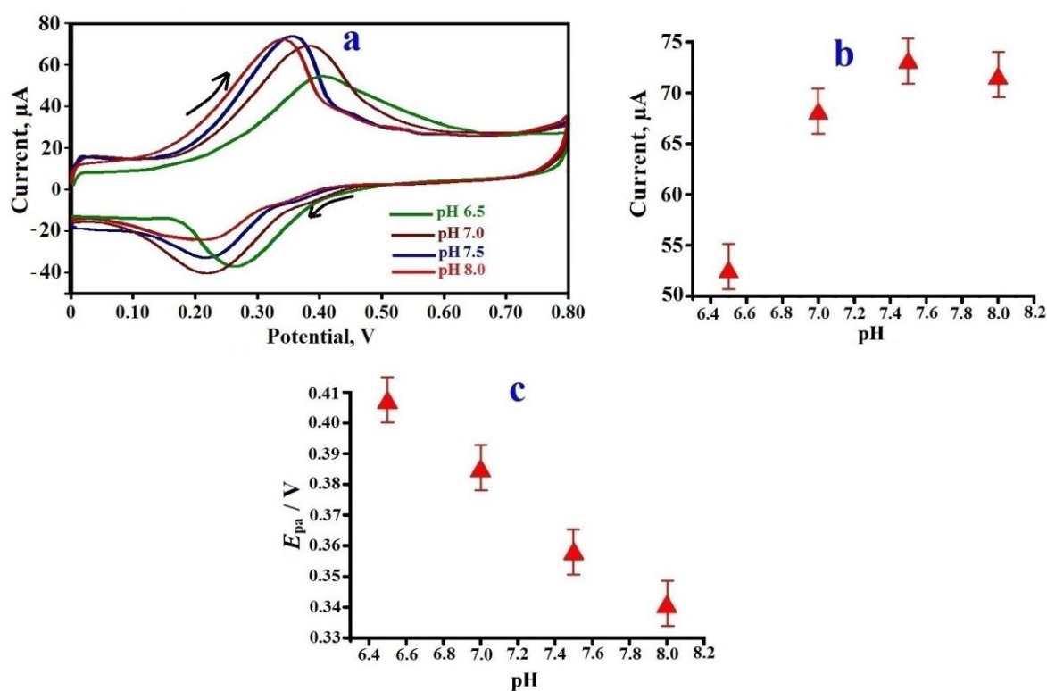
Figure 5: (a) CVs of 1 \times 10^{-4} \text{ M} PC at PMMCNTPE in 0.2 M PBS at pH varying from 6.5-8.0, at the scan rate 0.1 \text{ V s}^{-1} , (b) I_{pa} vs. pH dependence, (c) E_{pa} vs. pH dependence
