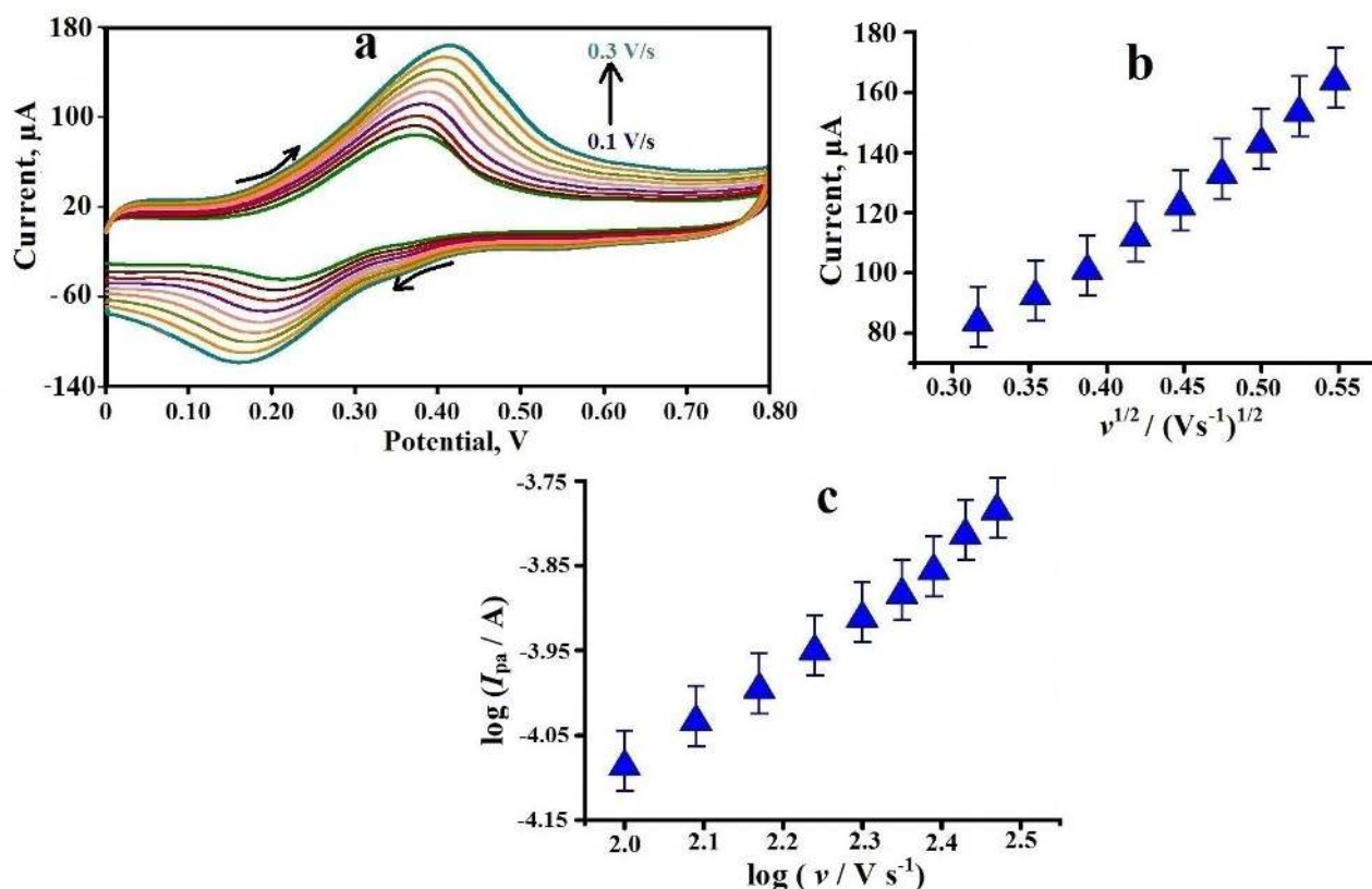
Figure 6: (a) CVs of 1 \times 10^{-4} M PC at PMMCNTPE in 0.2 M PBS of pH 7.5, recorded at different scan rates ranging from 0.1-0.3 \text{V s}^{-1} (b) I_{pa} vs. square root of scan rate (c) \log I_{pa} vs. \log v dependence
