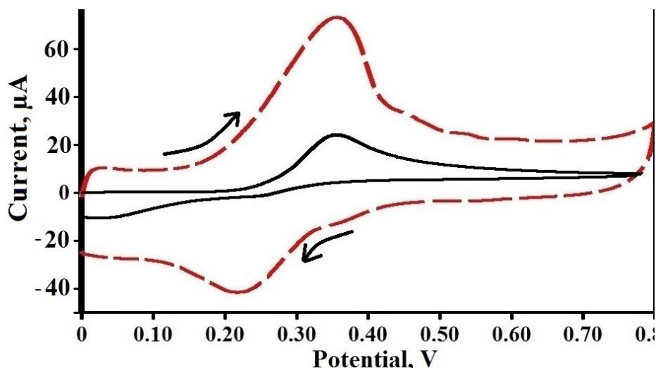
Figure 3. CVs of PC ( 1 \times 10^{-4} M ) at BCNTPE (solid line), and PMMCNTPE (dashed line) in 0.2 M PBS of pH 7.5, at the scan rate 0.1 \text{ V s}^{-1}
