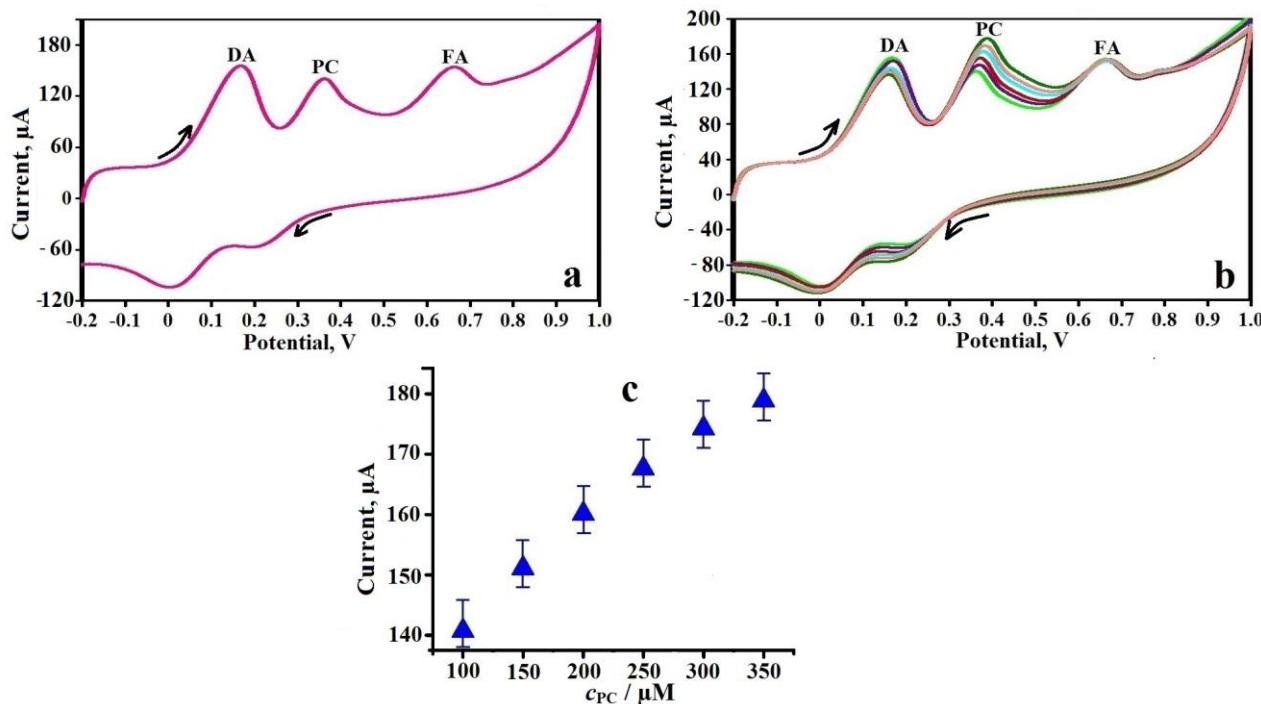
Figure 9. CV at PMMCNTPE in 0.2 M PBS of pH 7.5, recorded at the scan rate 0.1 \text{ Vs}^{-1} in presence of: (a) PC ( 1 \times 10^{-4} \text{ M} ), DA ( 1 \times 10^{-4} \text{ M} ) and FA ( 1 \times 10^{-4} \text{ M} ), (b) DA ( 1 \times 10^{-4} \text{ M} ), FA ( 1 \times 10^{-4} \text{ M} ), and PC of varying concentration from 1 \times 10^{-4} - 3.5 \times 10^{-4} \text{ M} , (c) I_{pa} vs. concentration of PC.
