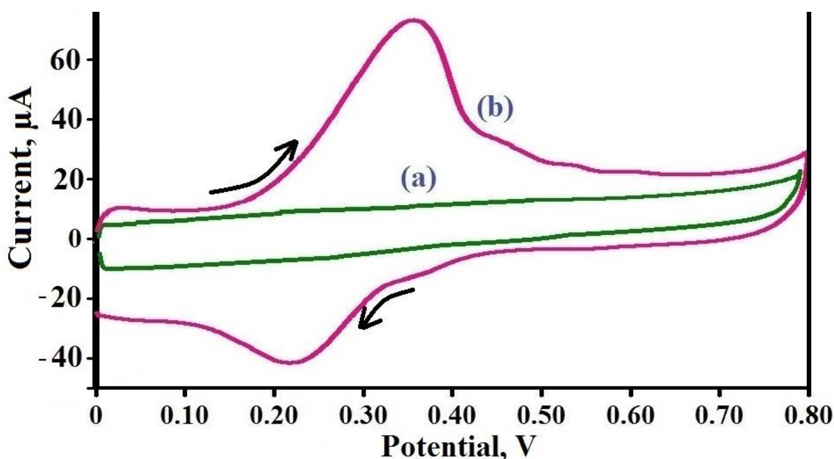
Figure 4. CVs of PMMCNTPE without PC (curve a) and with 1 \times 10^{-4} M PC (curve b) in 0.2 M PBS of pH 7.5, at the scan rate 0.1 \text{ V s}^{-1} .
