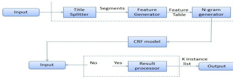
Fig. 2 Flow Chart of Title Classifier
