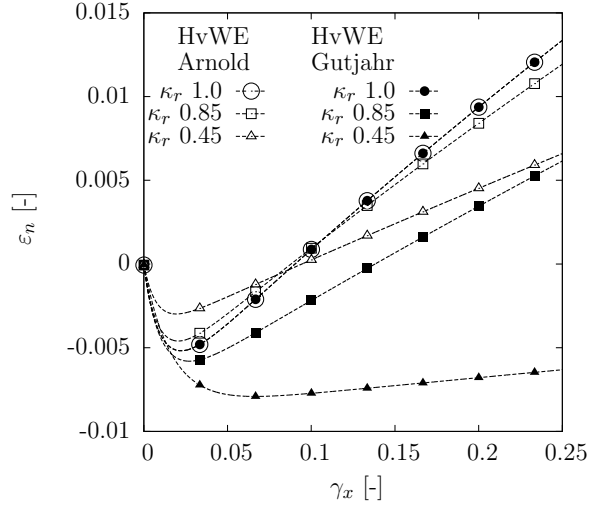
Figure 12: CNL simulation of the two different surface roughness modelling schemes in the \gamma_x - \varepsilon_x plot
