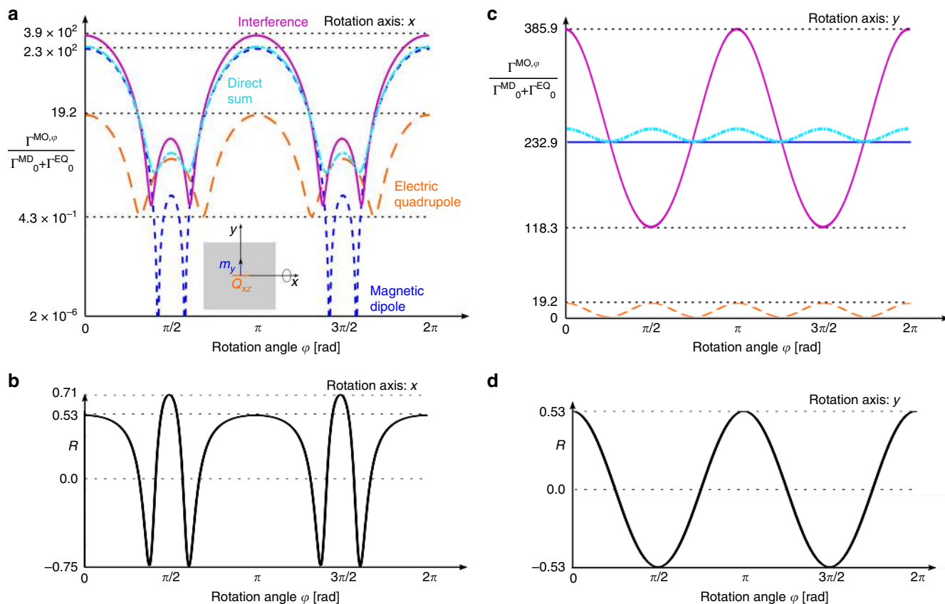
Fig. 3 Calculated transition rates and R parameters. Transition characteristics due to different multipolar mechanisms of a model \text{OsO}_3 molecule positioned in the center of the nanoantenna are shown in function of rotation angle with respect to x (a and b) or y axis (c and d). Original orientation of multipolar moments of transition 1 is depicted in the inset of panel (a). a Transition rates between the ground state 0 and excited state j = 1 . The magnetic dipole \Gamma^{\text{MD},\varphi} and electric quadrupole \Gamma^{\text{EQ},\varphi} contributions are shown with dotted blue and dashed orange lines, respectively. The total transition rate \Gamma (magenta solid line) includes the interference between the two contributing mechanisms, and may differ from their direct sum \Gamma^{\text{MD},\varphi} + \Gamma^{\text{EQ},\varphi} (cyan dash-dotted line). b Figure of merit R indicating the respective role of the interference terms for the full transition rate shown in (a). c, d As in panels (a), (b), but for rotations of the molecule around the y axis of the coordinate frame.
