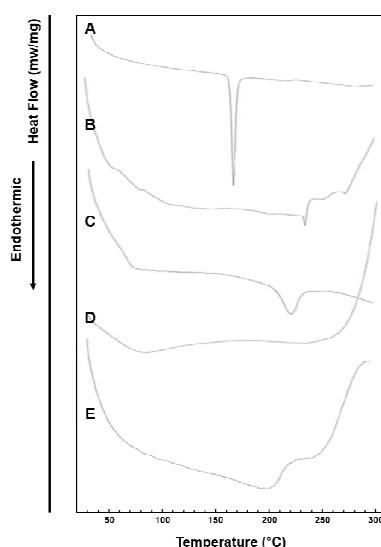
Figure 6. Differential scanning calorimetry (DSC) thermograms of (A) pure CLC, (B) PC, (C) Neusilin ® US2, (D) CCS, and (E) F11.
