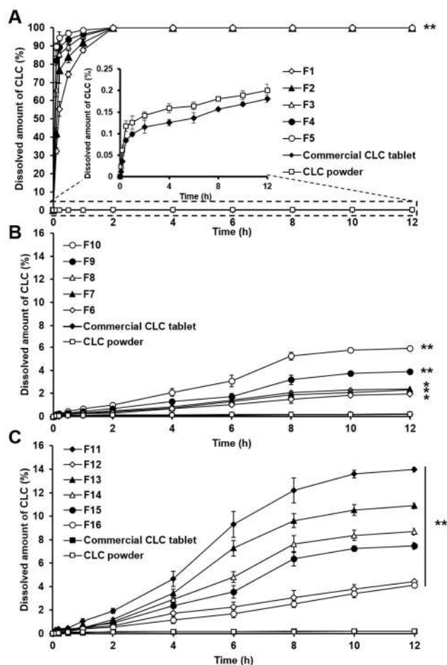
Figure 5. Dissolution profiles of CLC in water evaluated with (A) F1–F5, (B) F6–F10, and (C) F11–F16 for 12 h in comparison to those of commercial CLC 200 mg tablet and CLC powder. For clarity, the dissolution profiles of the commercial CLC tablet and CLC powder are expanded in the inserted graph in panel A. The dissolved amounts of CLC are presented as mean \pm SD ( n = 3 ) as a function of time up to 12 h. Single and double asterisks indicate the statistical differences in amounts of CLC dissolved at 12 h assessed with different PC-based dispersion formulations at P < 0.001 and P < 0.0001 , respectively, compared to that observed with the commercial CLC tablet. In panel A, all dissolved amounts of CLC were statistically greater than those of the commercial CLC tablet and CLC powder at P < 0.0001 marked with double asterisks.
