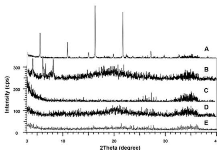
Figure 7. X-ray powder diffraction (XRD) patterns obtained from (A) pure CLC, (B) PC, (C) Neusilin ® US2, (D) CCS, and (E) F11.
