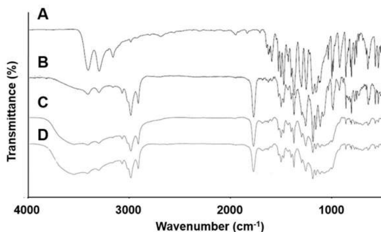
Figure 8. FT-IR spectra of (A) pure CLC, (B) F5 (CLC + PC), (C) F10 (CLC + PC + Neusilin ® US2), and (D) F11 (CLC + PC + Neusilin ® US2 + CCS).
