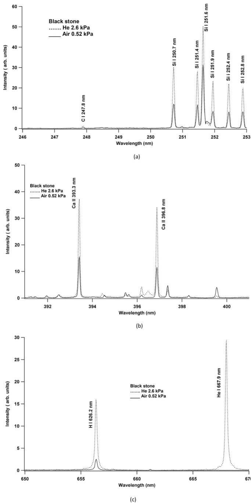
Fig. 4. Emission spectra measured from the plasma produced by focusing Nd:YAG laser beam of 60 mJ on a black stone in ambient He gas at 2.6 kPa and ambient air at 0.5 kPa; in the wavelength range of (a) 245 nm–255 nm, (b) 392 nm–400 nm and (c) 650–670 nm. The gate delay and gate width of the ICCD are set at 200 ns and 50 \mu s, respectively.
