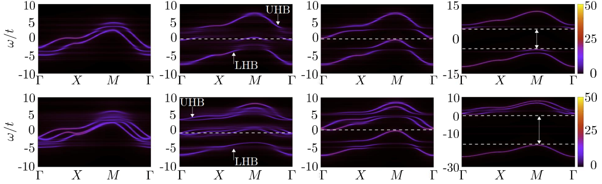
Figure 5: Evolution of the momentum-resolved spectral function obtained with DMFT upon increasing U and crossing the phase transition. First (second) row corresponds to N = 2 and \Omega/t = 0.5 ( N = 3 and \Omega/t = 0.4 ). From left to right, each panel corresponds to U \ll U_c , U \rightarrow U_c^- , U \rightarrow U_c^+ and U \gg U_c respectively. The specific values are U/t = 2, 6.9, 7, 16 in the first row, and U/t = 2, 6.9, 7, 24 in the second. UHB (LHB) in the second column from the left indicates the (precursor of the) Upper Hubbard Band (Lower Hubbard Band).
