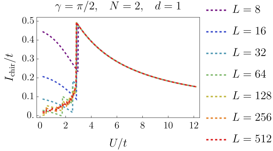
Figure 6: Finite-size scaling of the chiral current obtained by the Hartree-Fock method with \Omega = 0.4 t . The plot shows the case N = 2 , d = 1 , which is representative of all the other cases studied in this work.
