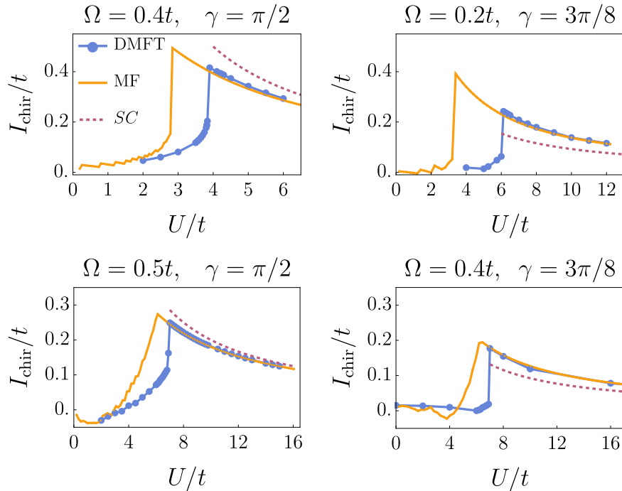
Figure 3: Chiral current as a function of the interaction U/t for a (1 + 1)-dimensional structure (first row) and a (2 + 1)-dimensional structure (second row); both for N = 2 (left column) and N = 3 (right column). The curves represent results obtained with different methods: a static mean field approach (MF), dynamical mean field theory (DMFT) and an effective strong-coupling limit (SC). All the techniques confirm the presence of a non differentiable peak in the function I_{\text{chir}}(U) at the transition and a 1/U tail in the insulating phase.
