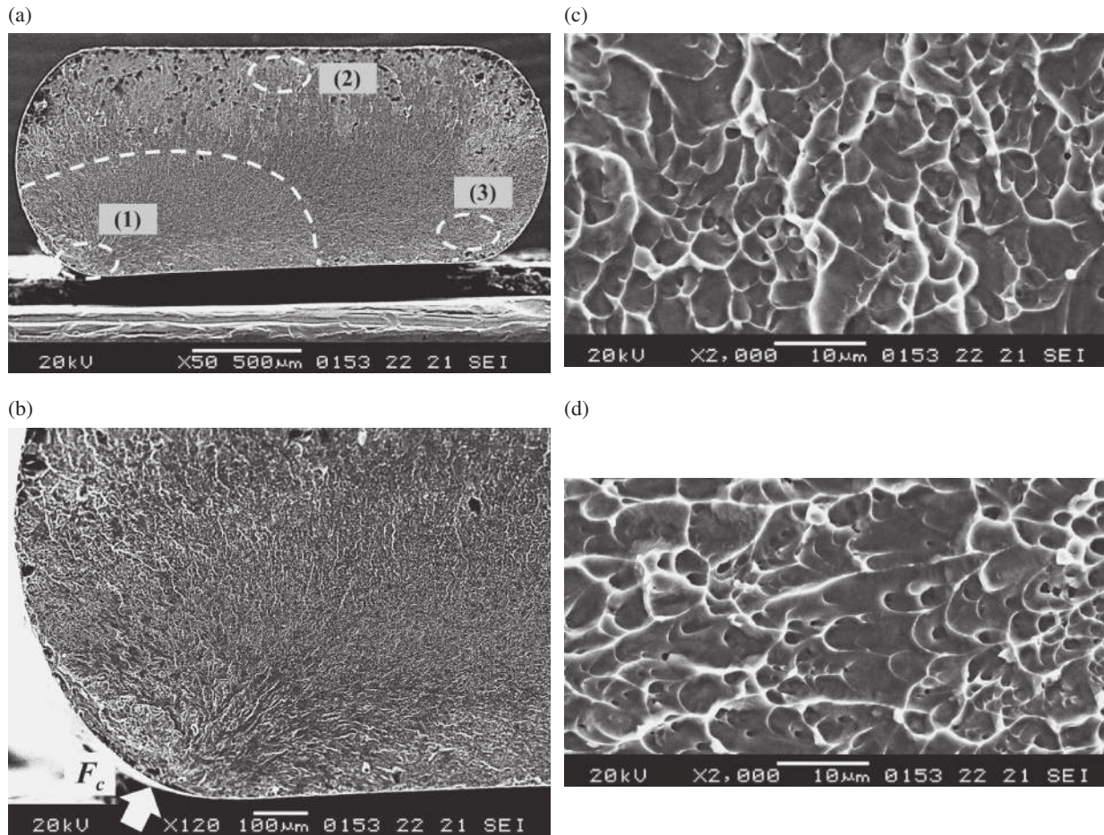
Fig. 5 SEM photographs of fracture surface of USP tape with d = 0.8 mm and c = 4000\% for \varepsilon_a = 1.64\% and N_f = 6788 : (a) whole fracture surface, (b) crack initiation part (1), (c) middle part of unstable fracture (2), and (d) final unstable fracture part (3).
