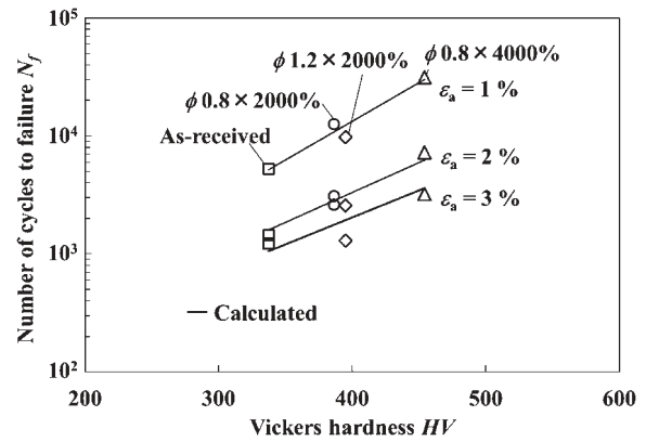
Fig. 9 Relationship between number of cycles to failure and Vickers hardness for various strain amplitudes \varepsilon_a .
