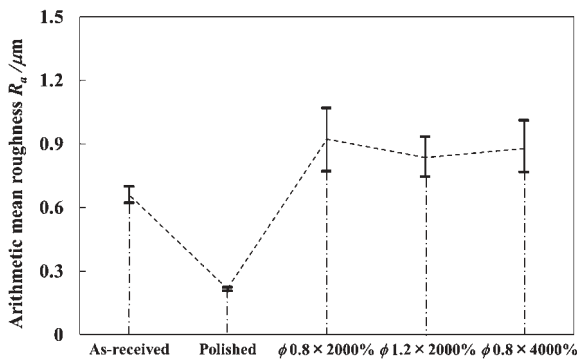
Fig. 10 Arithmetic mean surface roughness for five kinds of tapes.
