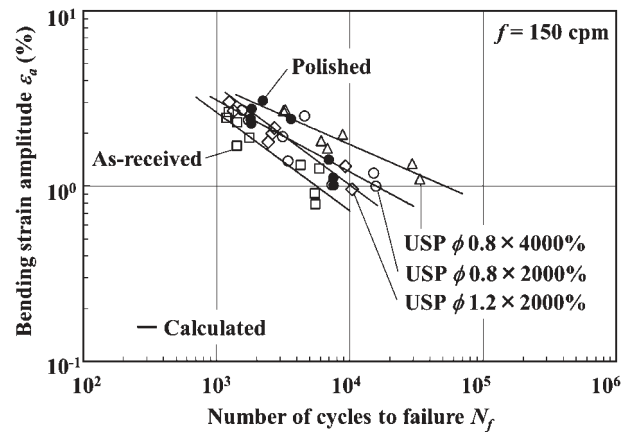
Fig. 2 Relationship between bending strain amplitude and the number of cycles to failure.
