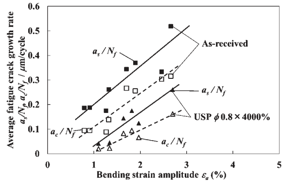
Fig. 8 Dependence of average fatigue crack growth rates a_s/N_f and a_c/N_f on bending strain amplitude \varepsilon_a for as-received tape and USP tape with d = 0.8 mm and c = 4000\% : a_s/N_f is shown by closed symbols and a_c/N_f by open symbols.
