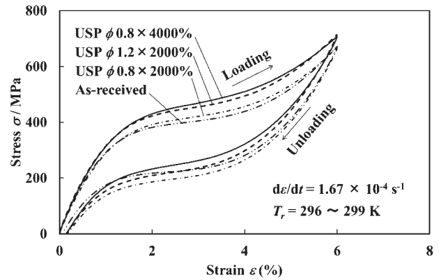
Fig. 1 Stress-strain curves.
