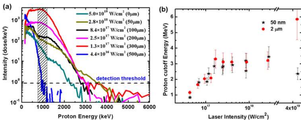
FIG. 2. (Color online) (a) Energy spectra of proton beams for 50 nm Al foils vs. laser intensities (focal offsets) for low contrast ( 10^{-6} ) laser pulses. Laser energy is kept as constant. (b) The E_{cutoff} of proton beams vs. varied focal intensities for 50 nm (black star) and 2 \mu m (red dot) foils.
