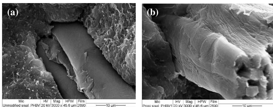
Figure 4. SEM micrographs of cross-section of (a) unmodified sisal/PHBV and (b) propionylated sisal/PHBV.
