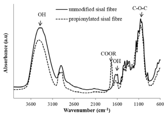
Figure 2. FTIR spectra of unmodified and propionylated sisal fibre.
