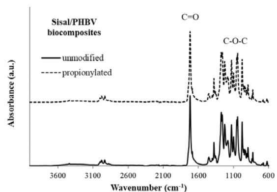
Figure 1. FTIR spectra of sisal fibre/PHBV biocomposites.
