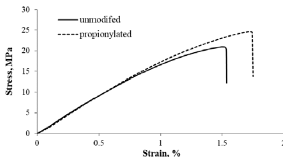
Figure 3. Stress-strain curve relationship of unmodified and propionylated sisal/PHBV biocomposites.
