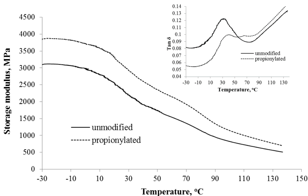
Figure 6. DMTA spectra (a) unmodified sisal/PHBV and (b) propionylated sisal/PHBV.
