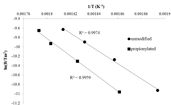
Figure 5. Relationship between \ln\left(\frac{\beta}{T_m^2}\right) and \left(\frac{1}{T_m}\right) using FWO method.
