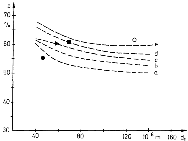
Fig. 6. Simulated floc void volume ε for different floc sizes d p and different interparticle distances δ for cubic packing. a: δ = 0; b: δ = 0.1; c: δ = 0.2; d: δ = 0.3; e: δ = 0.4 (10 -6 m). ● - experimental values for Ca 2+ bound flocs; ► - experimental values for P 20,000 bound flocs; ■ - experimental values for BPA 1,000 bound flocs; ○ - experimental values for Magna Floc LT25 bound flocs
