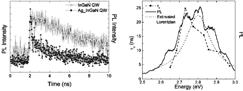
FIG. 2. (a) TRPL decay of the unsilvered and silvered InGaN QW for a 25-nm-wide wavelength detection window (2.79–2.96 eV), with pump energy of 3.14 eV. (b) Comparison of the time-integrated PL and the TRPL-measured recombination rate constant ( \tau_0 ) of the unsilvered InGaN QW. The dashed curve is the estimation given by Eq. (4) with \hbar\omega_c = 2.8 eV and \hbar\Delta\omega = 0.16 eV.
