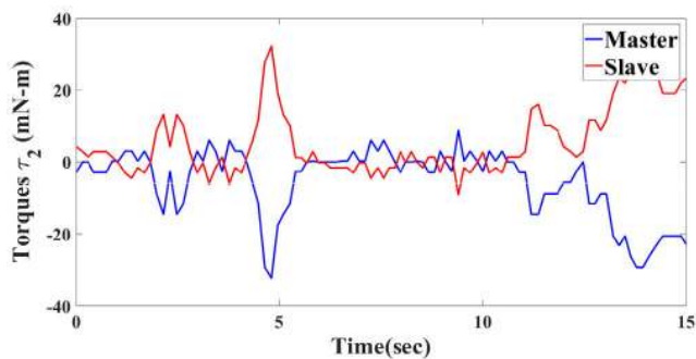
(c) Master and slave joint 2 torques
