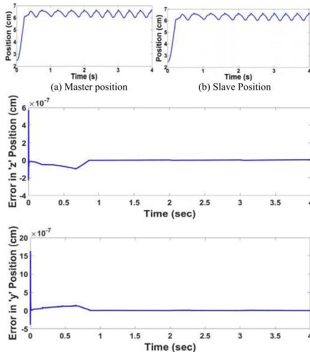
FIGURE 20. System retaining stability with zero-convergence using isotropy based design.
