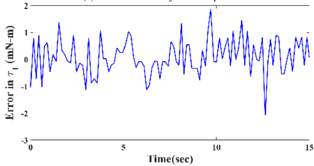
(b) Error in joint 1 torques
