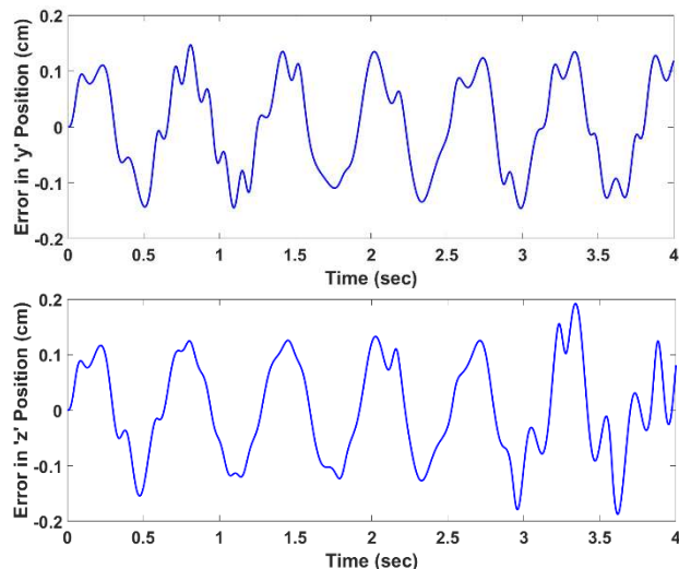
FIGURE 19. System retaining stability without zero convergence using state-of-art [9] controller.
