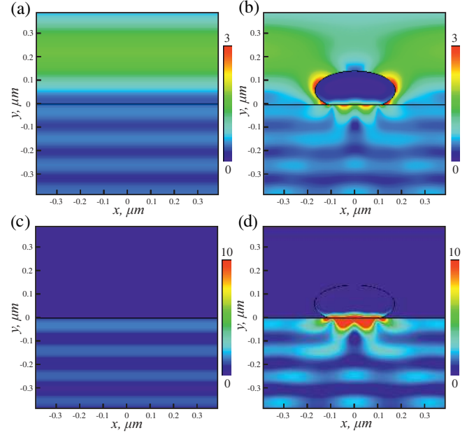
Figure 8 Numerically calculated electric field distribution profiles at the interface between air and the GaAs substrate (a) without and (b) with a silver nanoparticle. Densities of the power absorbed in the GaAs substrate (c) without and (d) with a silver nanoparticle.
