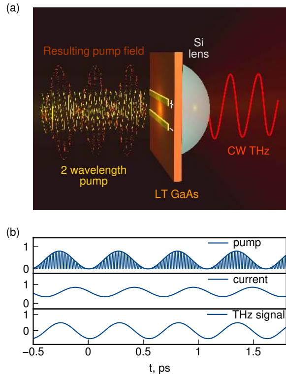
Figure 4 (a) Schematic illustration of CW THz generation by a LT-GaAs based photomixer and (b) time evolution of pump radiation envelope, antenna photocurrent and generated THz signal.
