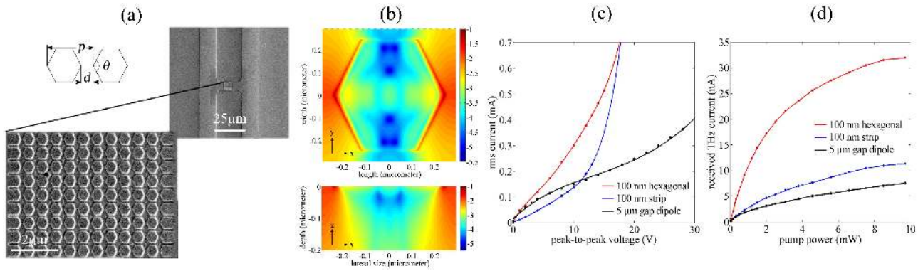
Figure 11 (a) SEM image of periodic array (with period p ) of hexagonal NAs arranged on a Si-GaAs substrate. (b) Electric field distribution profile near the hexagonal NA. (c) Peak-to-peak voltage dependence of photo-excited current in the hybrid THz antenna with hexagonal NAs (red curve), strip plasmonic gratings (blue curve), and the conventional dipole antenna (black curve). (d) Comparison of received THz currents from the hybrid THz antennas with hexagonal monopoles, strip plasmonic gratings, and conventional dipole antenna in depends on the pump optical power. [74]
