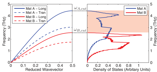
FIG. 1. (Color online) Phonon dispersion in the [100] direction and DOS of materials A and B calculated using harmonic lattice dynamics. The difference in cutoff frequencies is shown with respect to both the dispersion relationship and DOS. The red region demonstrates the vibrational mismatch and shows the density of phonon states in material A that do not exist in material B.
