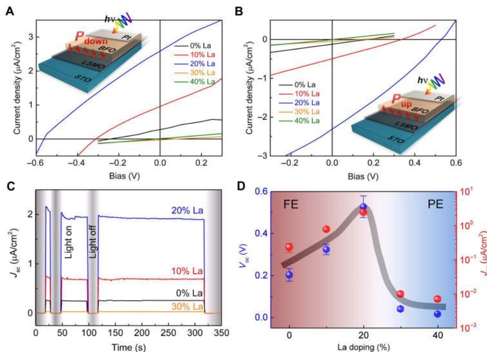
Fig. 2. Enhancement of photovoltaic effect of BFO by La substitution. Current density–voltage characteristics of La-substituted BFO films with (A) downward and (B) upward polarization states, respectively. The insets illustrate the device structure under test. (C) Time-dependent J_{sc} of different La-substituted BFO films. (D) Dependence of V_{oc} and J_{sc} on the La concentration, showing the progressive enhancement when approaching the phase transition boundary.
