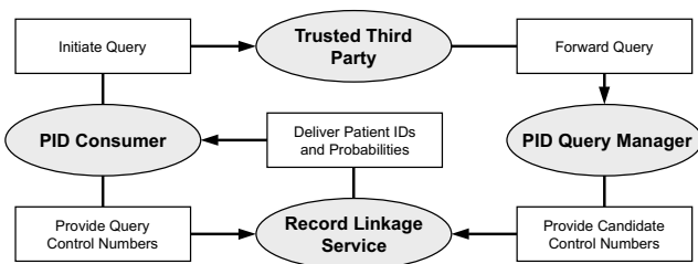
Fig. 11. Actors and Transactions in the PID Protocol (simplified)
