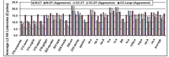
Figure 10. Average L2 hit latencies with the different schemes.
