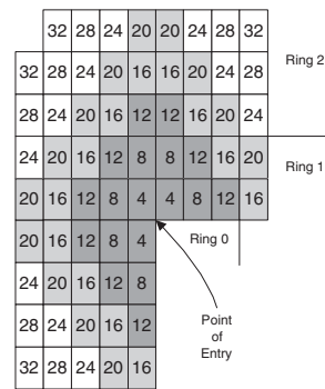
Figure 4. Layout of the preferred cells and access latencies as seen from a core’s perspective.
