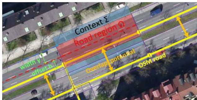
Figure 2. Illustration of the road centerline with the width parameterized by the center offset h and symmetrical width y . The direction and length of the rectangle \Omega_i is defined by the p_i, p_{i-1} points given by the street database. The context is depicted as \Sigma .
