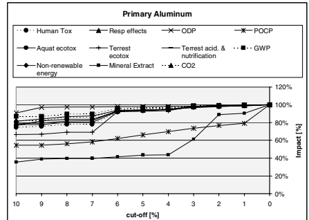
Figure 2-13: Analysis of cut-offs for primary aluminum
