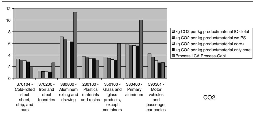
Figure 2-22: Comparison of results of reduced input-output LCA with process LCA (the various input-output results ("kg CO2 per .." differ due to different levels of exclusion of service related commodities, since their selection is not unambiguous)
