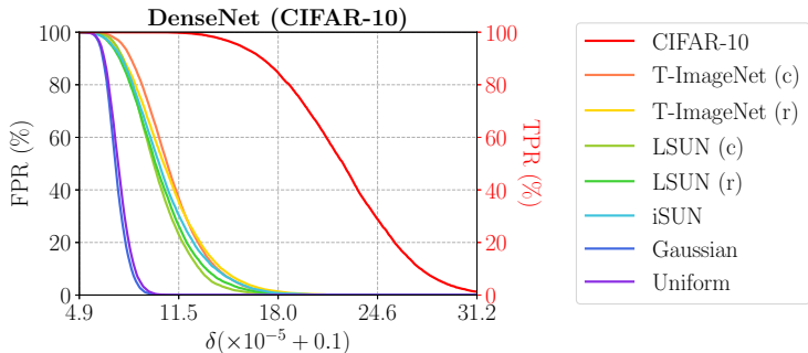
Figure 13: False positive rate (FPR) and true positive rate (TPR) under different thresholds ( \delta ) when the temperature ( T ) is set to 1,000 and the perturbation magnitude ( \varepsilon ) is set to 0.0014. The DenseNet is trained on CIFAR-10.
