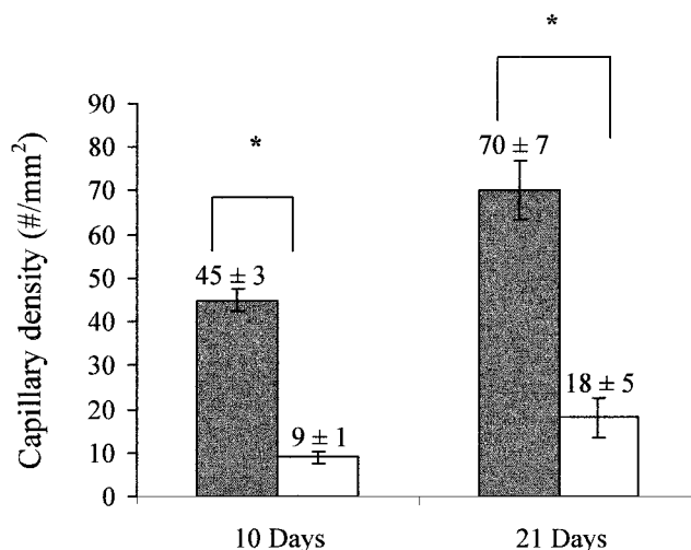
Figure 3. Kinetics of scaffold vascularization after implantation on the mesenteric membrane in rat peritoneum. Blood vessel density (number per \text{mm}^2 ) was determined in 15 different fields per each time point, randomly selected from captured images of three H&E slides per one animal, using Image Pro 3.0. Each group consisted of three animals. *The difference between the two groups for each time is significant (analysis of variance, single factor; p = 0.000013 for p < 0.01 ).
