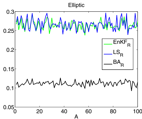
Figure 2. Comparison over different subspaces \mathcal{A} , generated from draws from the prior, of the relative errors of one iteration of \text{EnKF}_R versus (Tikhonov regularized) least squares ( \text{LS}_R ) and the best approximation ( \text{BA}_R ).
