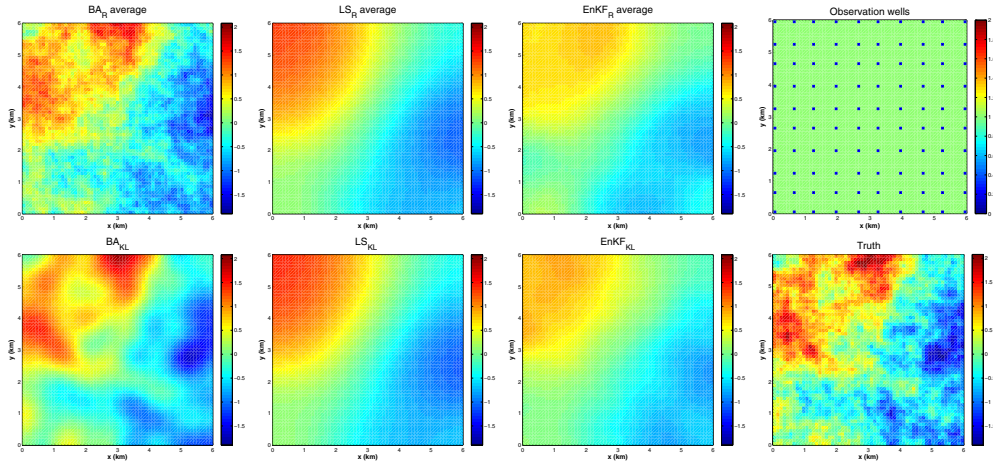
Figure 5. Estimated \log K . Top left: BA_R , average. Top middle left: LS_R , average. Top middle right: first iteration of EnKF_R , average. Top right: measurement well locations. Bottom left: BA_{KL} . Bottom middle left: LS_{KL} . Bottom middle right: EnKF_{KL} . Bottom right: the truth u^\dagger .
