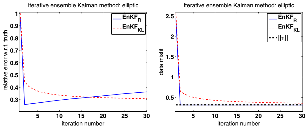
Figure 1. Performance of \text{EnKF}_R and \text{EnKF}_{KL} . Left: relative error with respect to the truth. Right: data misfit.
