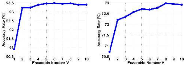
Figure 2: From left to right: The effects of ensemble number V on CIFAR10 and CIFAR100, respectively. The results are obtained by tuning different ensemble number V with \lambda = 0.1 .
