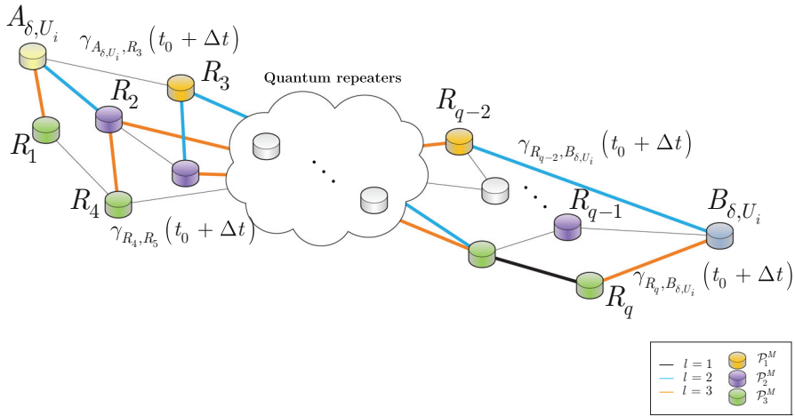
Fig. 2 A quantum Internet setting with m = 3 connection-disjoint entangled paths \mathcal{P}_1^M , \mathcal{P}_2^M and \mathcal{P}_3^M between an i th source quantum node A_{\delta, U_i} and target quantum node B_{\delta, U_i} with demand \rho , and q intermediate R_i quantum repeaters, i = 1, \dots, q . The entangled paths consist of l = 1 level (direct) and multilevel, l = 2, 3 level entangled connections. The quantum nodes of \mathcal{P}_1^M are depicted by orange, the nodes of \mathcal{P}_2^M by purple, and the nodes of \mathcal{P}_3^M by green. The \gamma_{x,y}(t_0 + \Delta t) coefficients are derived for all entangled connections of the paths
