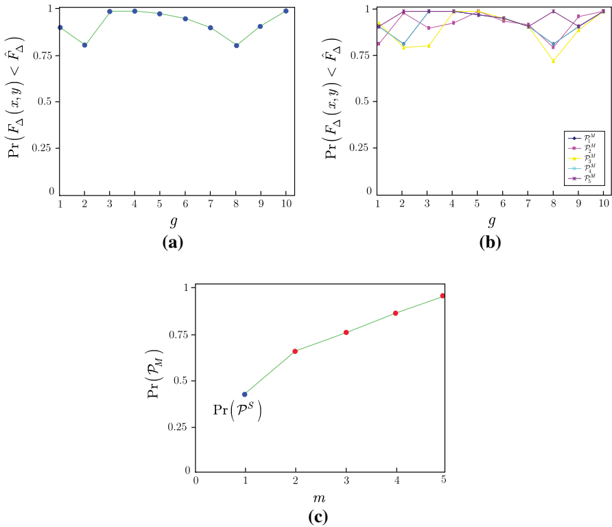
Fig. 3 The probability of shared entanglement between the source and the destination with the fidelity criterion at a single entangled path and at a multipath setting, F_{\text{crit}} = 0.98 , \hat{F}_{\Delta} = 0.02 , g_S = g = 10 . a A distribution of the \Pr F_{\Delta}(x, y) < \hat{F}_{\Delta} probabilities for the g entangled connections of a \mathcal{P}^S single path. b A distribution of the \Pr(F_{\Delta}(x, y) < \hat{F}_{\Delta}) probabilities for the g_S = g entangled connections of a \mathcal{P}_M = \{\mathcal{P}_1^M, \dots, \mathcal{P}_m^M\} multipath setting, m = 5 . c The \Pr(\mathcal{P}_M) probabilities in function of m . The \Pr(\mathcal{P}_S) single-path probability is yielded at m = 1
