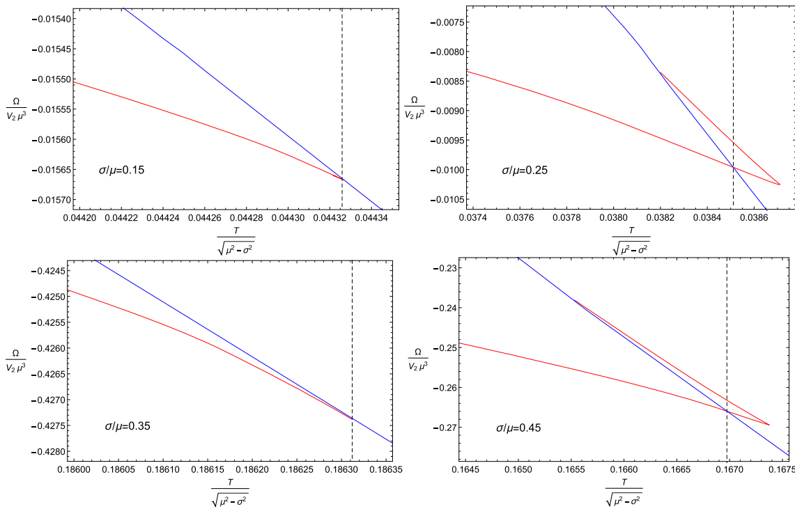
Fig. 2 the free energy \Omega as a function of the temperature T for operators \mathcal{O}_{+} (top two panels) and \mathcal{O}_{-} (bottom two panels) with the strength of the backreaction \gamma = 0.2 . In each panel, the red lines and blue
