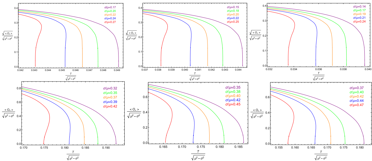
Fig. 1 The condensates \langle O_{+} \rangle and \langle O_{-} \rangle in terms of temperature in the backreacted holographic superfluid model. The left two panels are for the backreaction \gamma = 0.1 , the middle ones are for \gamma = 0.2 , and the right ones are for \gamma = 0.3
