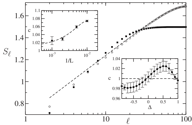
FIG. 7. The block entropy S_\ell for L=200 in the case of an XXZ Heisenberg chain for a critical value \Delta=0.0 (circles) and non-critical value \Delta=1.8 (squares). The critical data compared with the conformal field theory prediction (dashed line). Lower inset: Central charge extrapolated by fitting the numerical data S_\ell with Eq. (42) (with a factor 1/2 as done in the numerical calculation with the block at the boundary) for different values of \Delta . The data are for L=1000 . Upper inset: Scaling of c extrapolated as a function of 1/L for the worst case \Delta=0.5 and compared to a quadratic fit (dashed line). From De Chiara et al. , 2005 .
