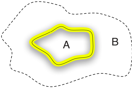
FIG. 6. (Color online) The block entropy is evaluated after partitioning the system in regions A and B . For finite range correlations, it is intuitive that the wave function of the system is factorized |\Psi_A\rangle|\Psi_B\rangle by removing the region at the boundary. Accordingly the reduced entropy would vanish.
