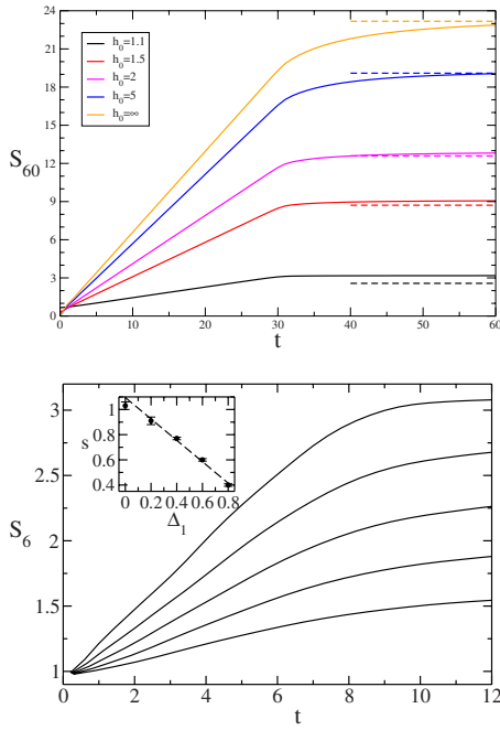
FIG. 28. (Color online) Evolution of the entropy for different types of quenches in the case of the Ising (top panel) [from Calabrese and Cardy (2005)] and Heisenberg (bottom panel) [from De Chiara et al. (2005)] models. The block are of 60 and 6 sites in the Ising and Heisenberg cases, respectively. In the Ising case the quench are obtained by changing the external magnetic field from h_0 to h_1=1 . In the Heisenberg model the anisotropy parameters are used instead, \Delta_0=1.5 while \Delta_1=0.0, 0.2, 0.4, 0.6 , and 0.8 . The time is expressed in units of the spin wave velocity. The inset of the top panel shows the behavior of the initial slope as a function of the final value of the anisotropy.
