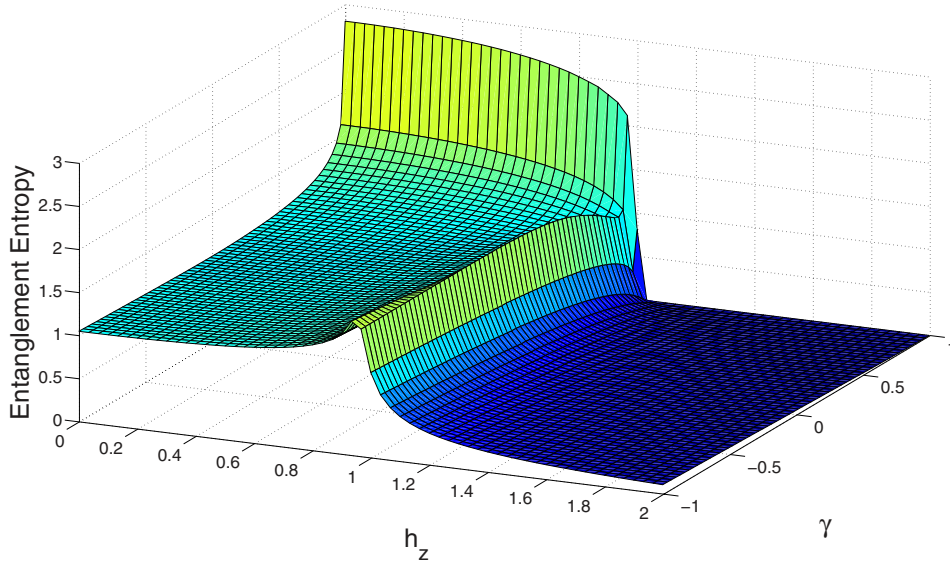
FIG. 12. (Color online) Entanglement entropy for N=500 and \ell=125 as a function of the parameters h_z and \gamma of the ferromagnetic LMG model. For \gamma \neq 1 , there is an anomaly at the critical point h_z=1 , whereas the entropy goes to zero at large h_z since the ground state is a fully polarized state in the field direction. In the zero field limit, the entropy saturates when the size of the system increases. For \gamma=1 , the entropy increases with the size of the system in the region 0 \leq h_z < 1 and jumps to zero at h_z=1 . From Latorre, Orus, et al., 2005 .
