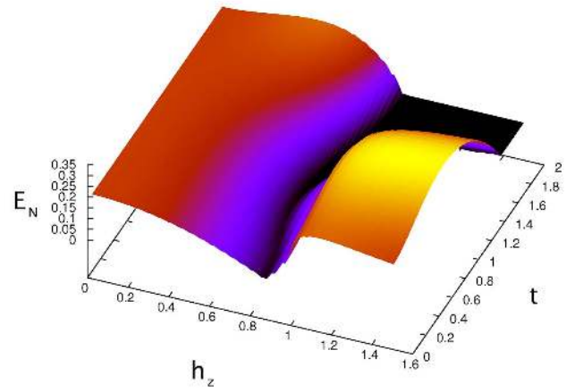
FIG. 27. (Color online) The nearest-neighbor logarithmic negativity E_N as a function of the initial transverse field h_z and time t for the anisotropy \gamma=0.5 . At short times t \leq 1.8 the dynamical phase transition is a point of reentrance for the entanglement. At later times the state remains separable for values of the field above the critical value. For t=0 , entanglement vanishes, as it should, as h_z grows. The transverse magnetization of the evolved state does not show a similar critical behavior as a function of h_z . From Sen(De) et al. , 2005.
