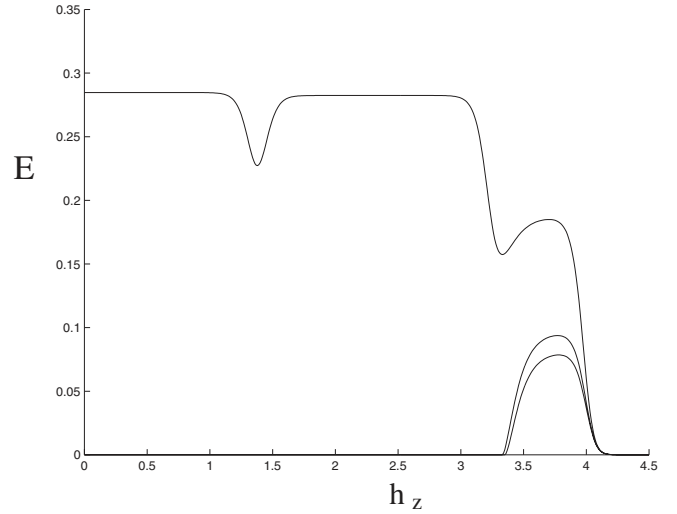
FIG. 16. Entanglement between two qubits interacting according to the antiferromagnetic Heisenberg model as a function of the external field h_z and temperature (multiplied by the Boltzmann's constant) T with coupling J=1 . The topmost plot shows the variation of nearest-neighbor entanglement with the magnetic field. The middle and bottommost plots show the same for next-nearest and next-to-next-nearest neighbors, respectively, from Arnesen et al. , 2001.
