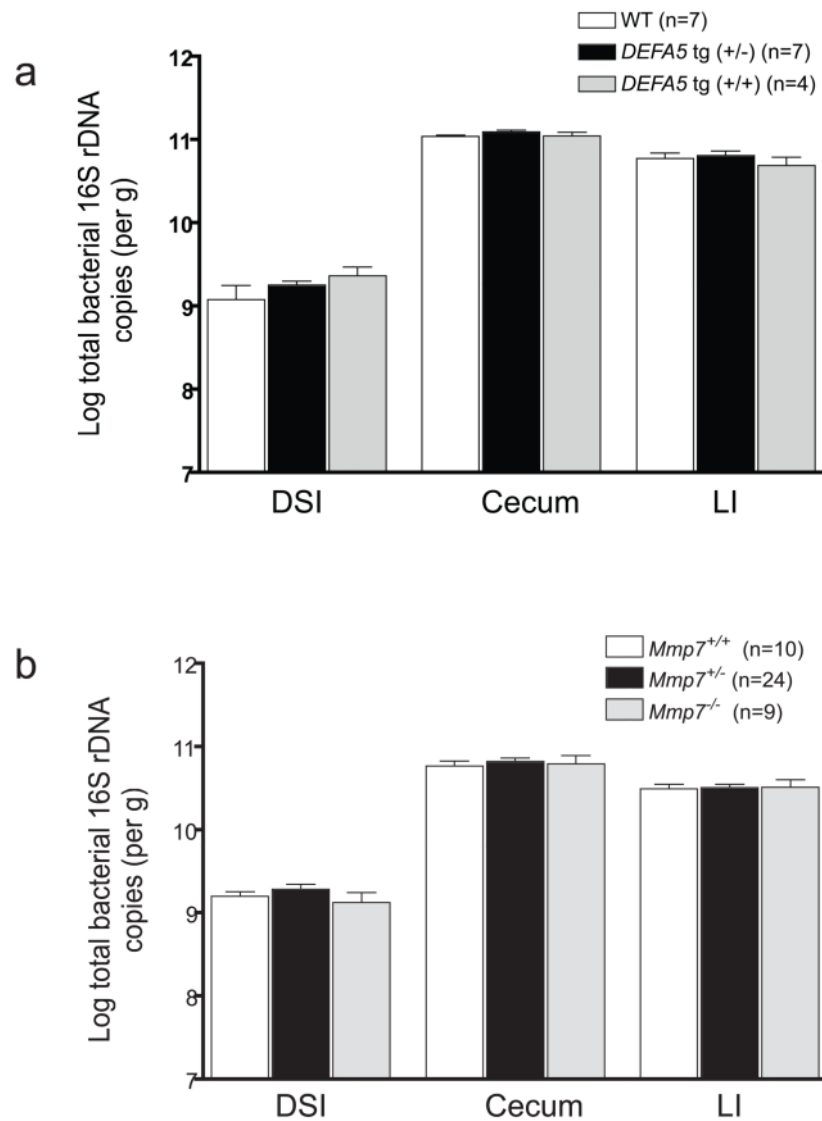
Figure 6. Quantitative comparison of total bacteria by intestinal segment. Log number of total copies of bacterial 16S rDNA were determined for distal small intestine (DSI), cecum, and large intestine (LI) of each mouse by qPCR, using universal bacterial primers, and quantified using a standard curve generated from Ruminococcus productus bacterial genomic DNA as a reference strain. Offspring from DEFA5 tg (+/-) (a) and Mmp7 +/- (b) breeding pairs were analyzed.
