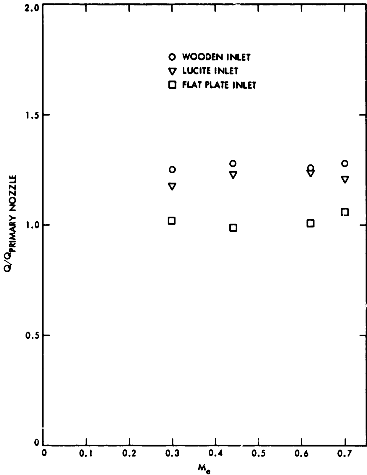
Figure 25. Influence of Ejector Inlet Flow on Entrainment
