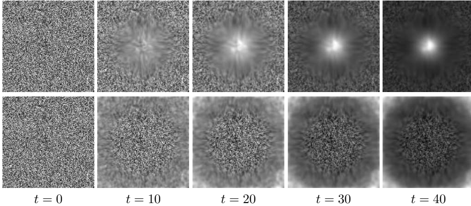
FIG. 4.6. Non-linear diffusion by gradient flow on the generalized entropies (4.4). Top row: fixed m_i = 1.4 and varying weights b_i \in [1, 20] (1 in the boundary, 20 in the center). Bottom row: fixed b_i = 1 and varying exponents m_i \in [1, 2] (1 in the boundary, 2 in the center).
