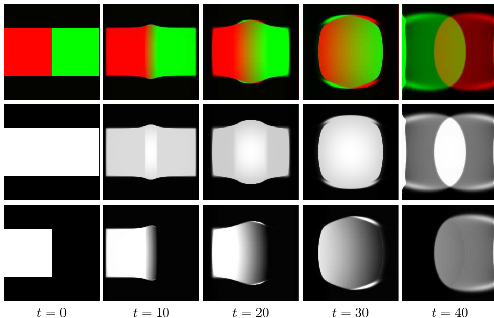
FIG. 5.4. Evolution with a summation coupling \iota_{[0,\kappa]}^N(p_1 + p_2) where \kappa = \|p_{1,t=0}\|_\infty = \|p_{2,t=0}\|_\infty . Top row: display of both p_{1,t} (red) and p_{2,t} (green), yellow indicates a mixing. Middle row: display of p_{1,t} + p_{2,t} . Bottom row: display of p_{1,t} .
