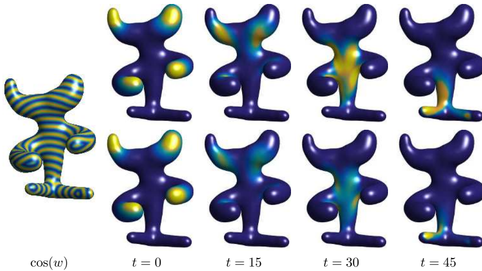
FIG. 4.3. Display of the evolution p_t on a triangulated surface. From top to bottom, the congestion parameter is set to \kappa/\|p_{t=0}\|_\infty \in \{1, 6\} .
