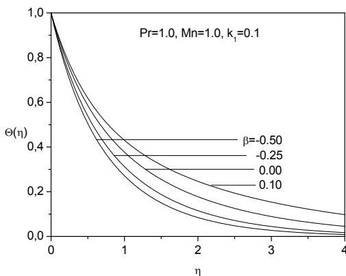
Fig. 7. Effect of the heat source/sink parameter on the temperature.
