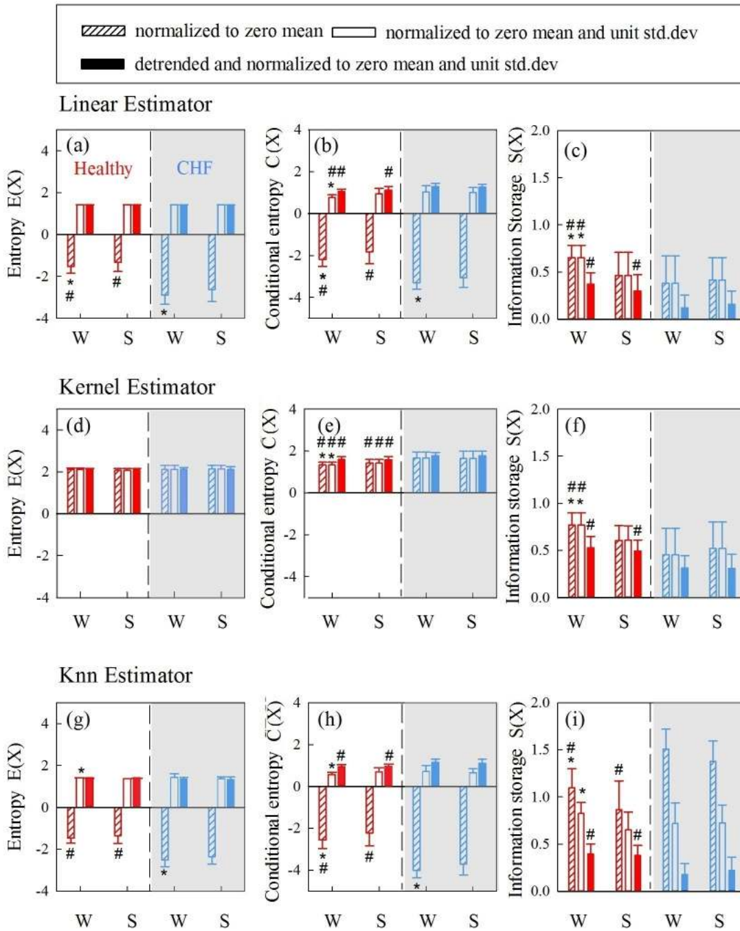
FIG. 22: Performance of entropy estimators and entropy measures for heart rate variability signals of healthy subjects and congestive heart failure (CHF) patients measured during wake (W) and sleep (S) states. Panels contain the behavior of entropy (a,d,g), conditional entropy (b,e,h) and information storage (c,f,i) computed for signals normalized to zero mean within each window (shaded bar), signals normalized to zero mean and unit standard deviation within each window (open bar) and signals detrended by a linear high-pass filter and normalized to zero mean and unit standard deviation within each window (solid bar) for healthy subjects (left side with white background and red bars) and CHF subjects (right side with grey background and blue bars) during wake (W) and sleep (S). Barplots depict the mean + standard deviation across subjects of the median value of entropy measures computed for consecutive windows of 300 data points with a 150 points overlap using m = 2 lagged components and implemented with the linear estimator (a-c), the kernel estimator with threshold r = 0.2 (d-f), and the knn estimator with k = 10 neighbors (g-i). Symbols denote statistical significance ( p < 0.05 ) of the differences between W and S (*, paired t-test) or between healthy and CHF (#, unpaired t-test). Results: Compared to healthy subjects, CHF patients exhibit lower Entropy values reflecting depressed HRV, and higher conditional entropy and lower information storage reflecting higher dynamical complexity. Healthy subjects display a day-to-night increase of the dynamical complexity (higher conditional entropy and lower information storage during S than during W) that is not observed in CHF patients.
