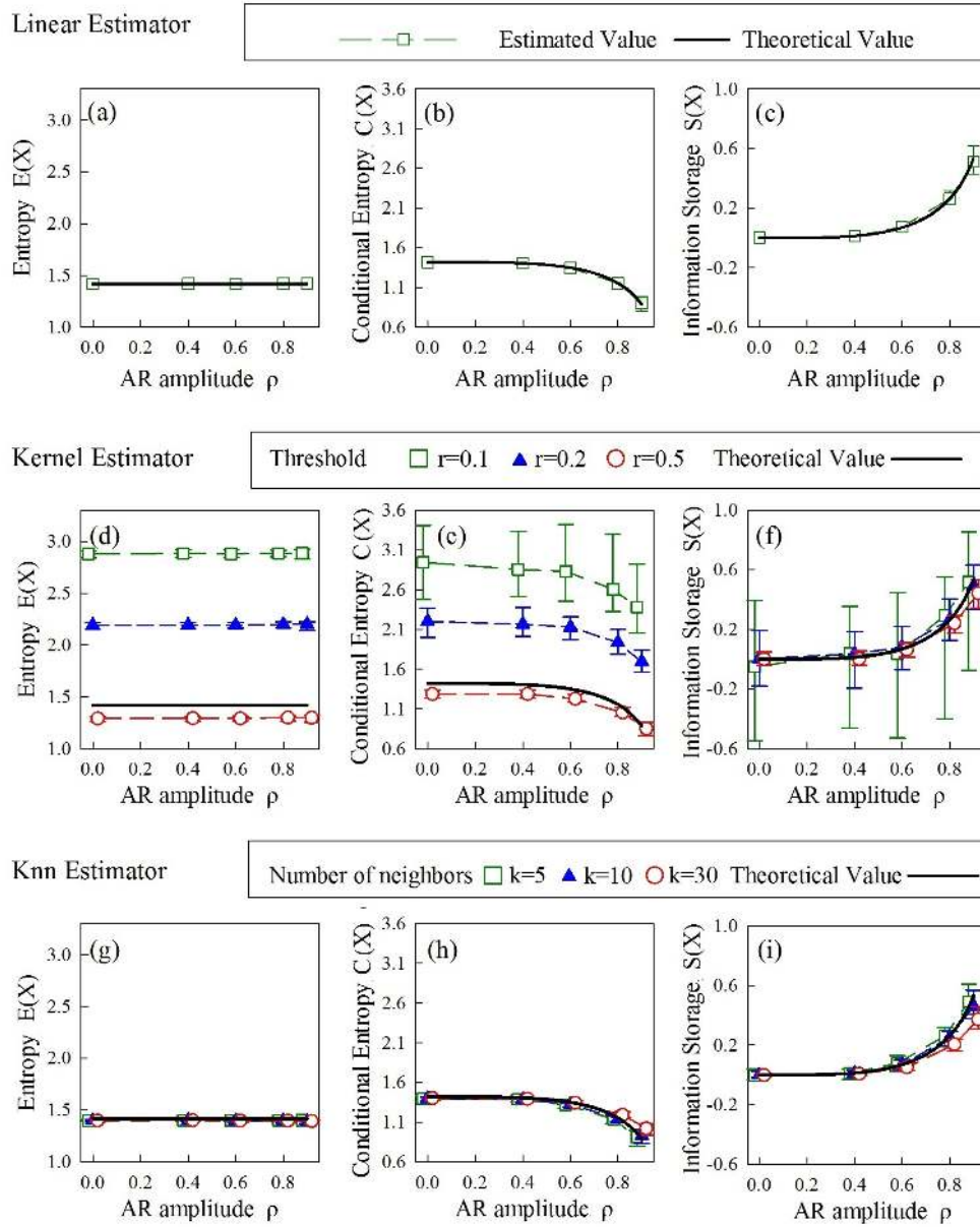
FIG. 9: Dependence of entropy estimators on estimator parameters for stationary AR processes. Plots depict the theoretical values (black solid line) and the estimated distributions (mean and 25% – 75% percentiles over 100 realizations, colored symbols and error bars) of entropy (a,d,g), conditional entropy (b,e,h) and information storage (c,f,i) computed using the linear estimator (a-c), the kernel estimator (g-i) implemented with threshold r = 0.1 (green open squares), r = 0.2 (blue full triangles) and r = 0.5 (red open circles), and the knn estimator (g-h) implemented with k = 5 (green open squares), k = 10 (blue full triangles) and k = 30 (red open circles) neighbors. Estimates are computed over realizations of length N = 300 , generated with fixed AR frequency f = 0.25 and varying the AR amplitude in the range \rho \in \{0, 0.4, 0.6, 0.8, 0.9\} . Results: The kernel estimates of entropy and conditional entropy are strongly dependent on the parameter r setting the kernel threshold, whereas the knn estimates are much less sensitive to the parameter k setting the number of neighbors. Since the linear estimator assumes the form of the probability distributions, it has no free parameters.
