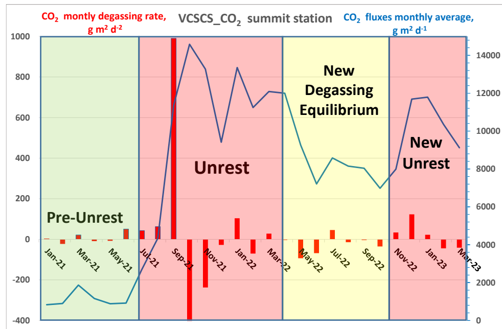
Figure 8. CO 2 fluxes monthly average (g m -2 d -1 ) blue line and CO 2 degassing rate (g m -2 d -2 ) red bars from January 2021 to March 2023.
